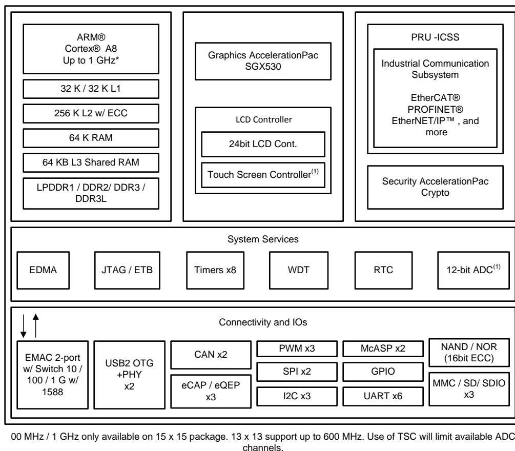
Figure 3. AM335x Block Diagram
