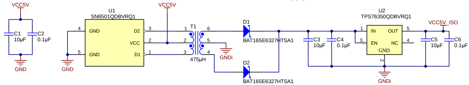
Isolated Power Supply
