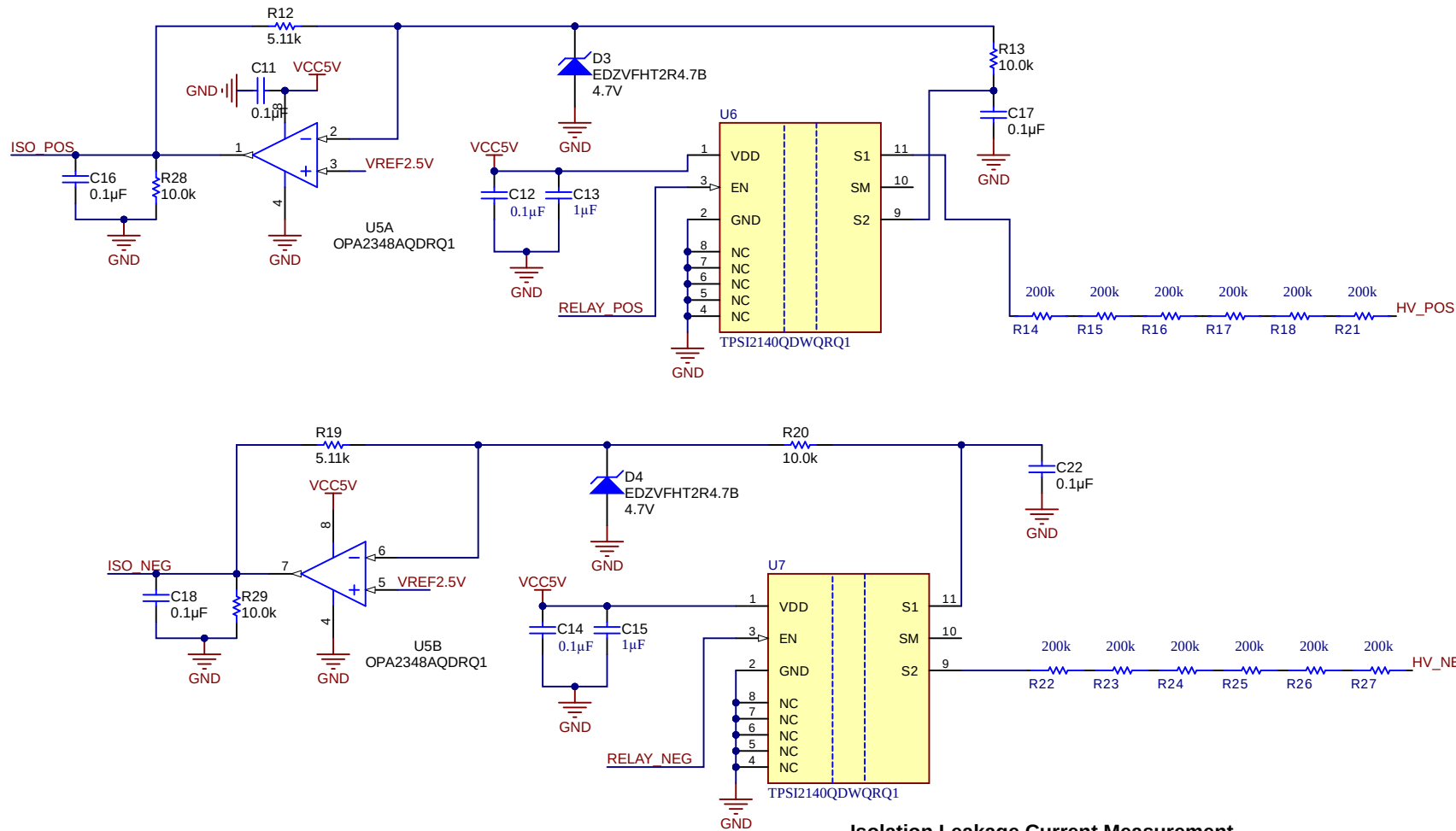
Isolation Leakage Current Measurement
