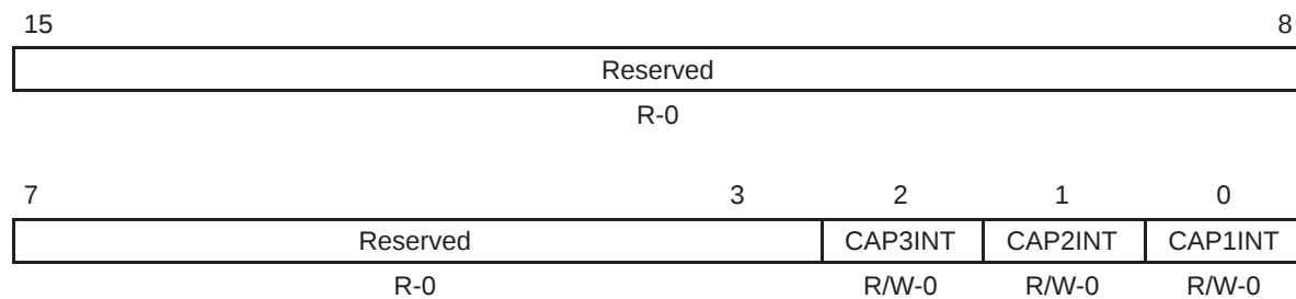
Figure 5–22. EVA Interrupt Mask Register C (EVAIMRC) — Address 742Eh
