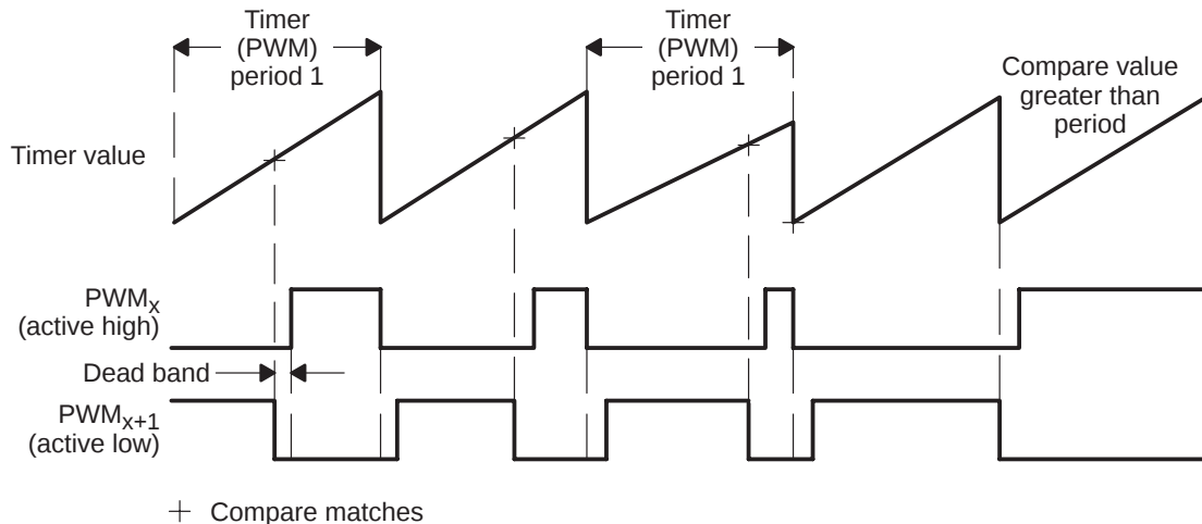
Figure 2-4. Asymmetric PWM Waveform Generation With Compare Unit and PWM Circuits ( x = 1, 3, \text{ or } 5 )
