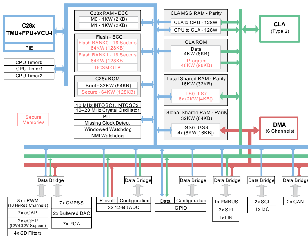
Figure 1. F28004x Functional Block Diagram
