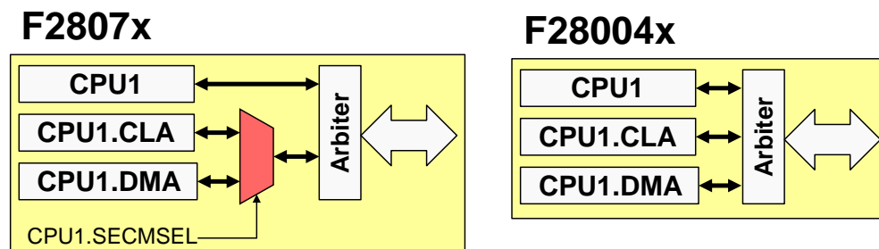
Figure 6. CPU/CLA/DMA Peripheral Access
