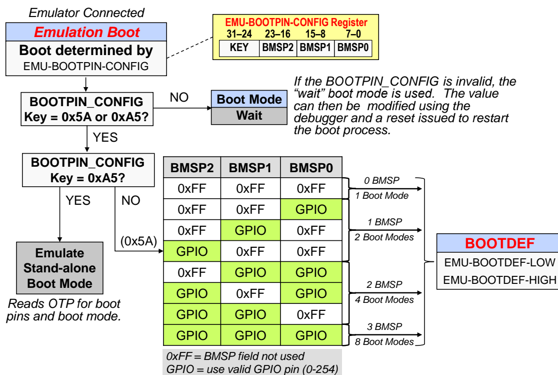
Figure 3. Emulation Boot Mode
