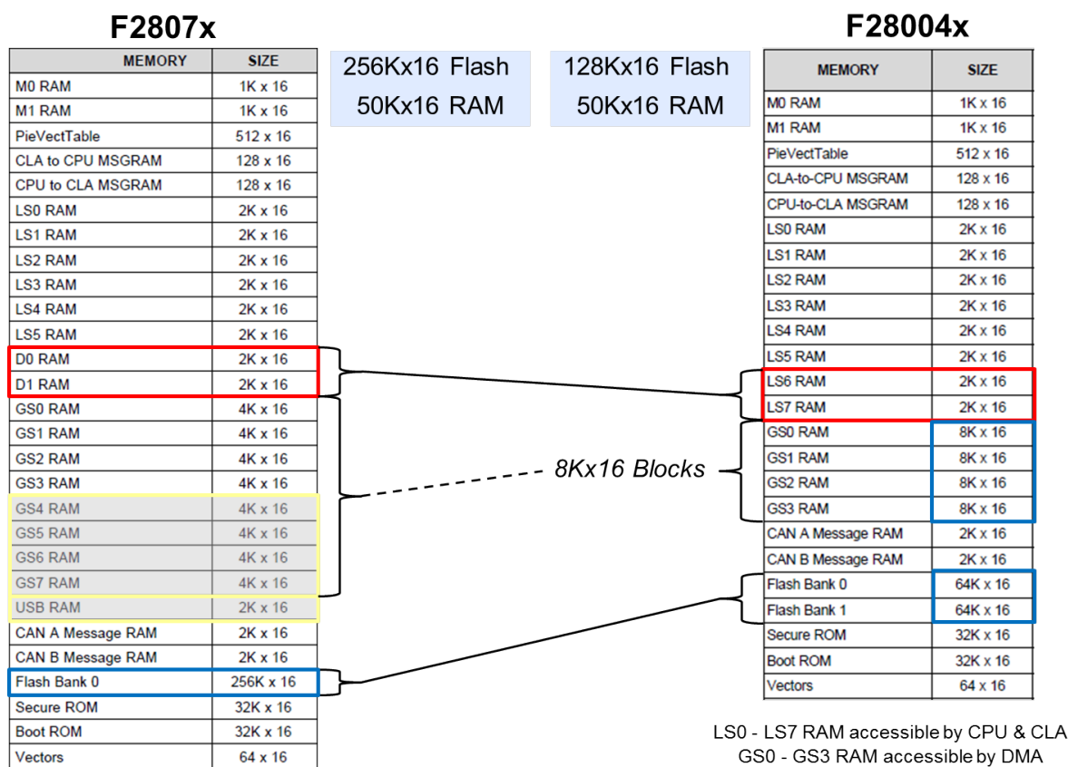
Figure 2. F28004x and F2807x Memory Map Comparison
