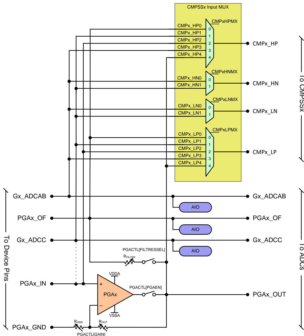
Figure 7. Analog Group Connections
