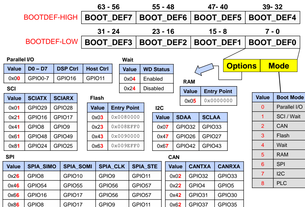
Figure 5. Boot Mode Definitions
