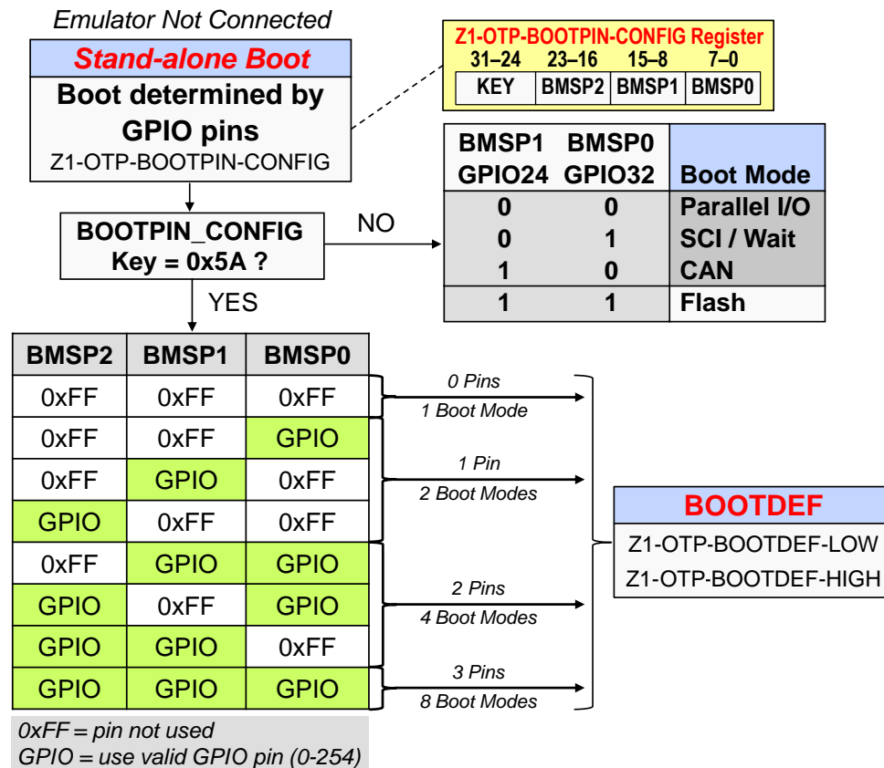
Figure 4. Stand-Alone Boot Mode
