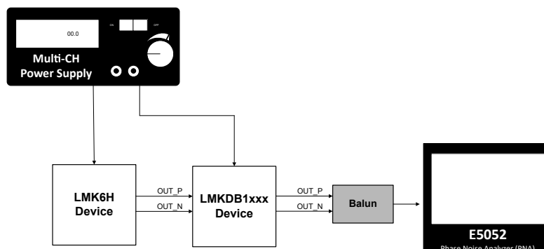
Figure 2-1. TI's PCIe Compliance Test Hardware Setup for Frequency Domain Measurements
