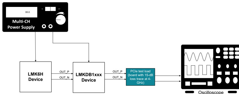
Figure 2-2. TI's PCIe Compliance Test Hardware Setup for Time Domain Measurements
