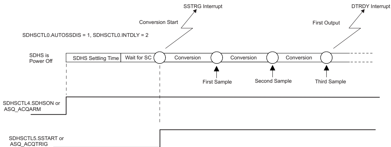
Figure 22-23. First Interrupt Position With SDHSCTL0.INTDLY = 2
