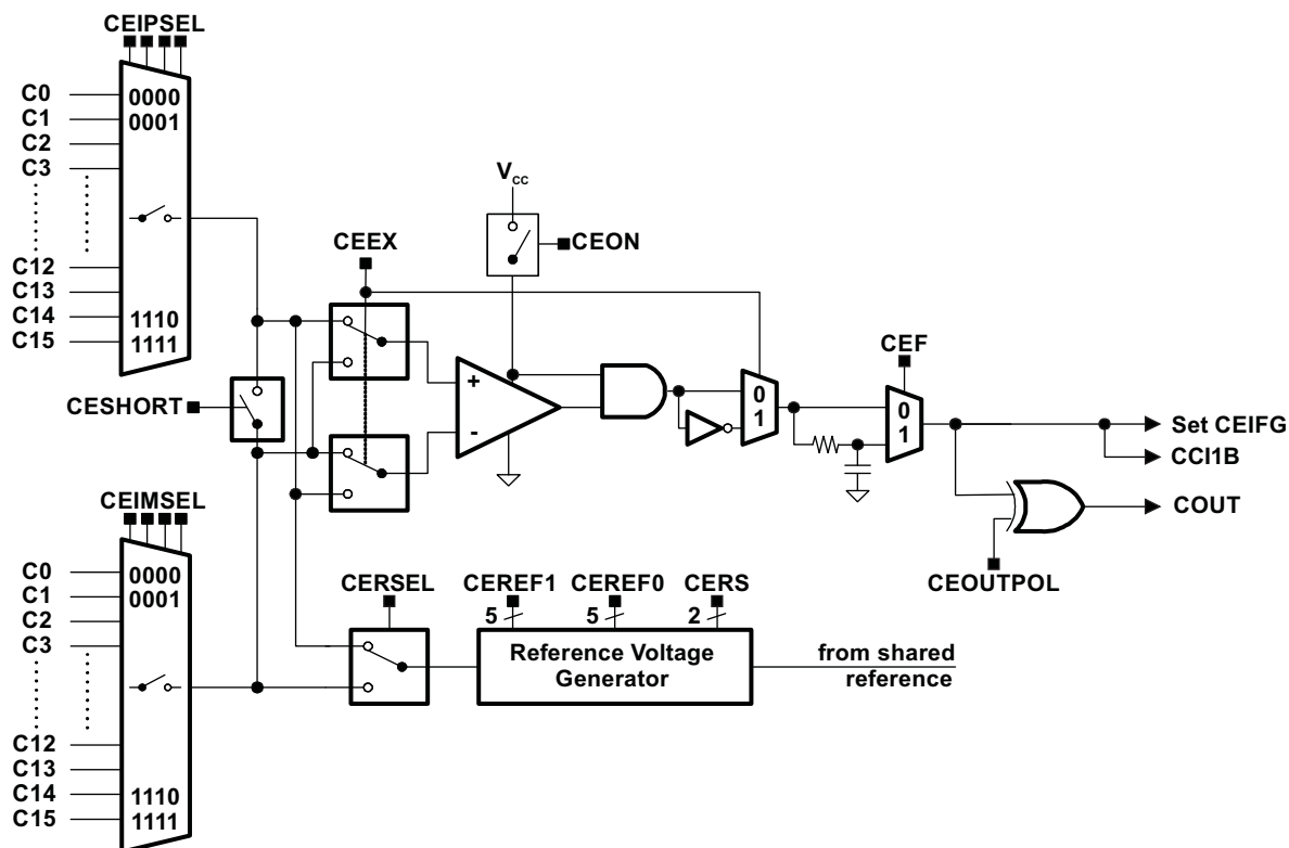
Figure 35-1. Comparator_E Block Diagram
