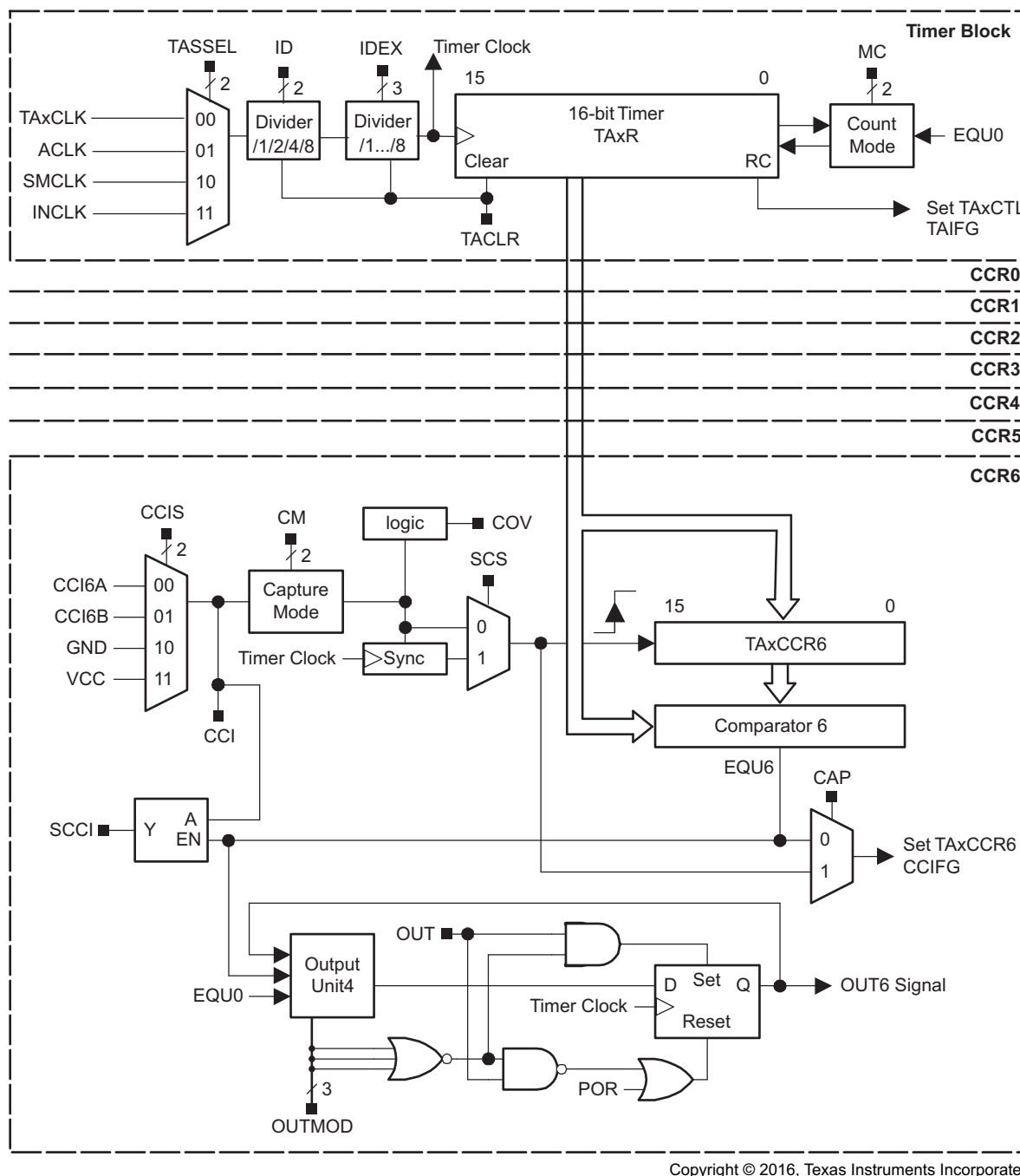
Figure 25-1. Timer_A Block Diagram
