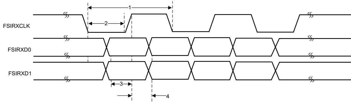
Figure 6-80. FSIRX Timings
