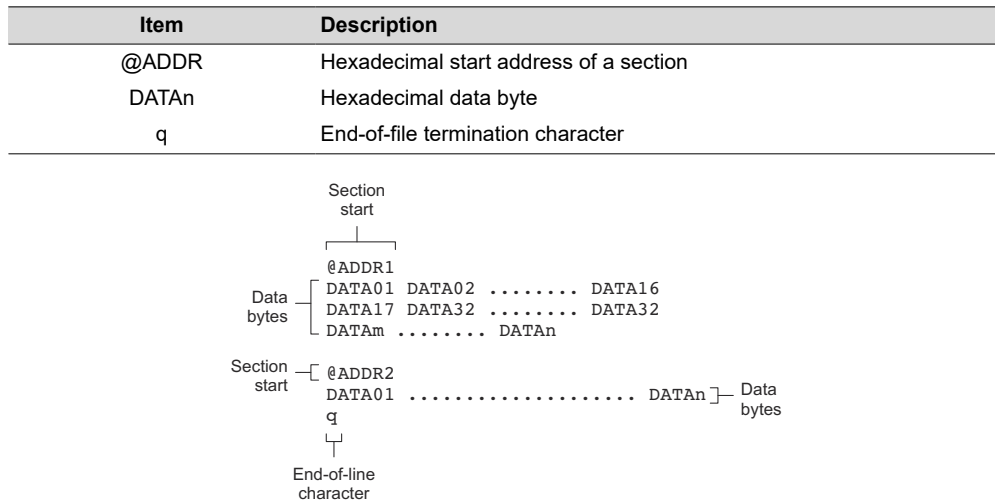
Figure 10-11. TI-TXT Object Format
