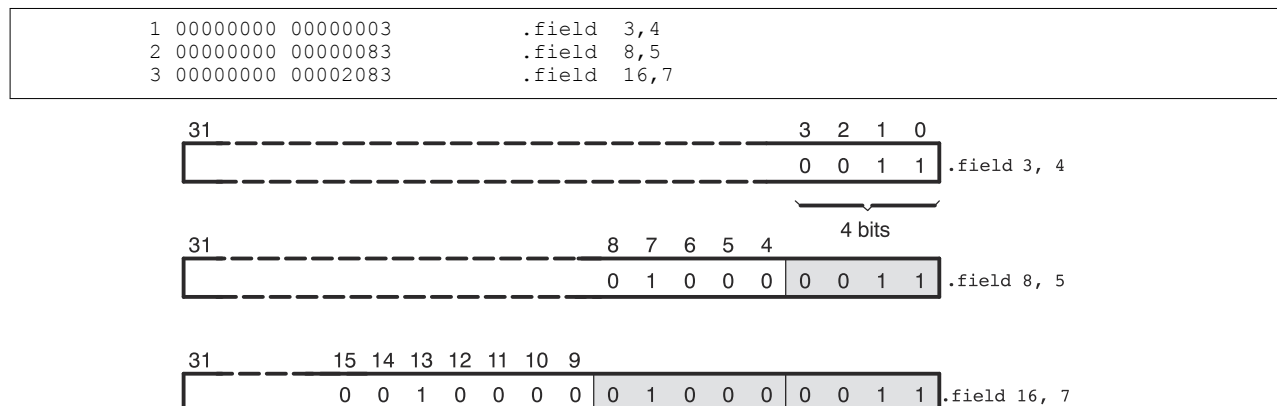
Figure 5-1. The .field Directive
