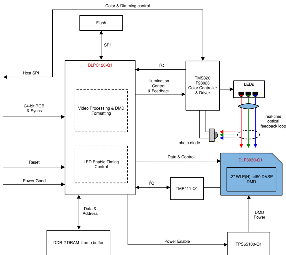
Figure 2-1. TIDA-080004 Block Diagram
