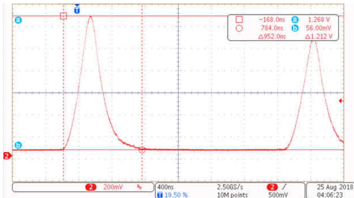
Figure 3-1. Shortest LED Pulse of 952 ns
