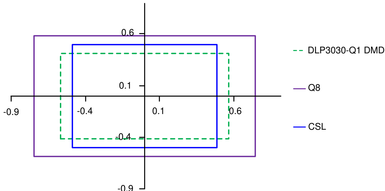
Figure 2-7. Etendue Diagram of 0.3" DMD With Different LEDs at f/2.4 Aperture
