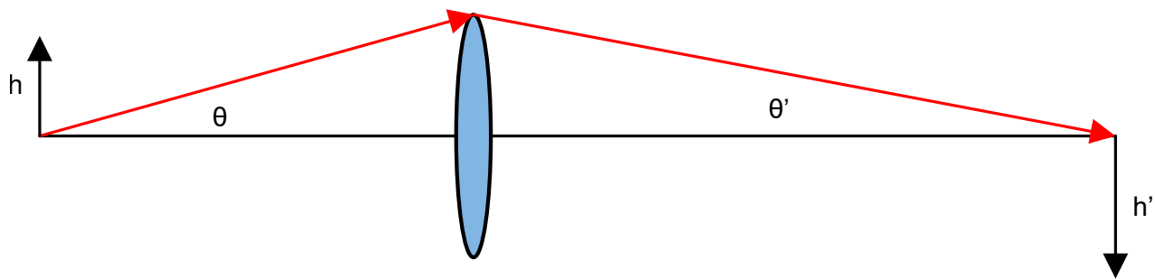
Figure 2-6. Abbe Sine Invariant Component Diagram
