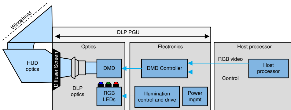
Figure 2-2. Head-up Display System Block Diagram
