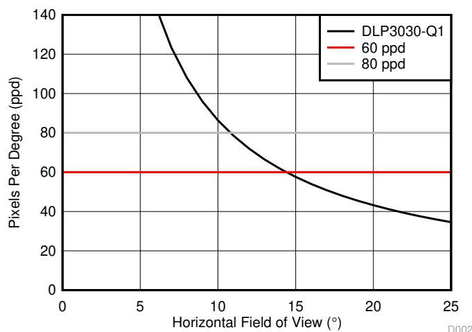
Figure 2-4. Resolution vs Field of View
