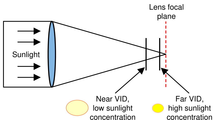
Figure 2-5. Increased Sunlight Concentration With a Longer Virtual Image Distance
