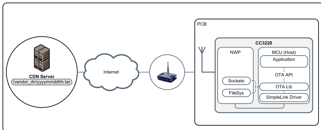
Figure 2-10. OTA System-Block Diagram
