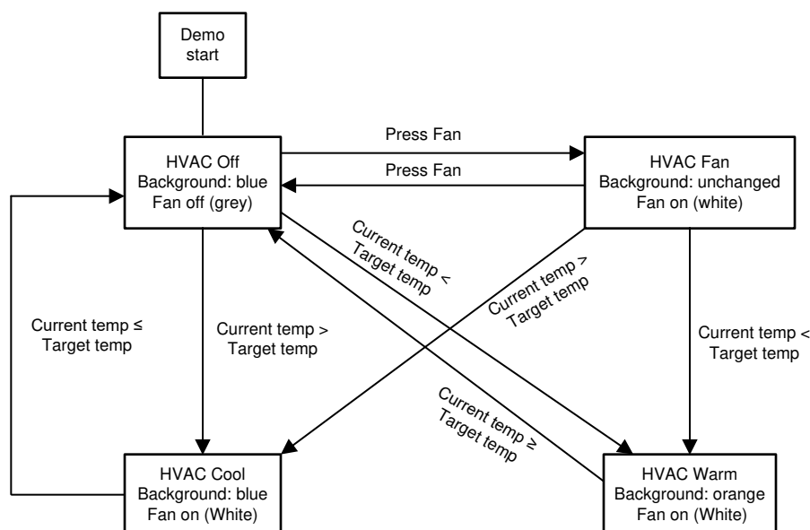
Figure 2-5. State Diagram of HMI Event Flow
