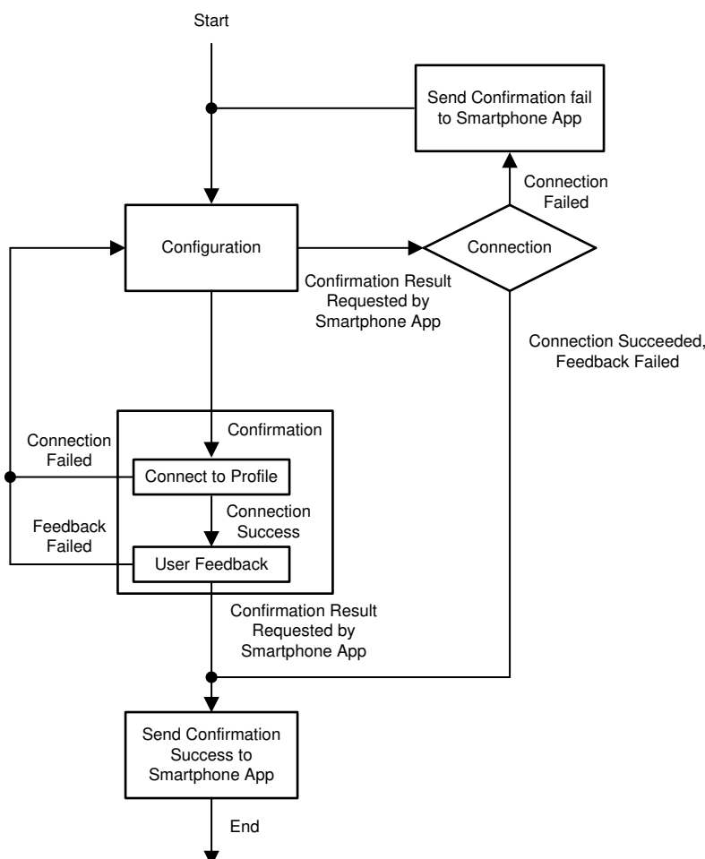
Figure 2-7. Provisioning-Process Flow Chart
