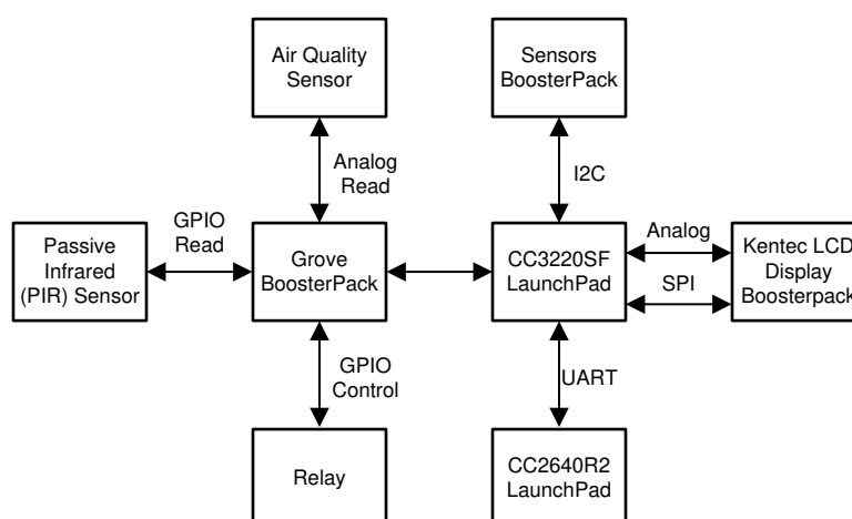
Figure 2-1. TIDM-1020 Block Diagram with BLE Provisioning
