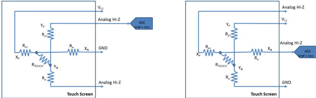
Figure 2-6. Configuration to Read XY Position of Touch Sensor
