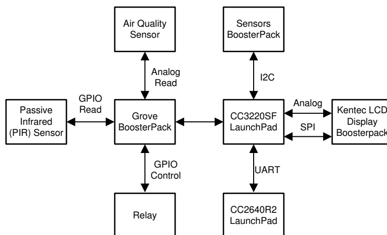
Figure 2-3. TIDM-1020 Block Diagram
