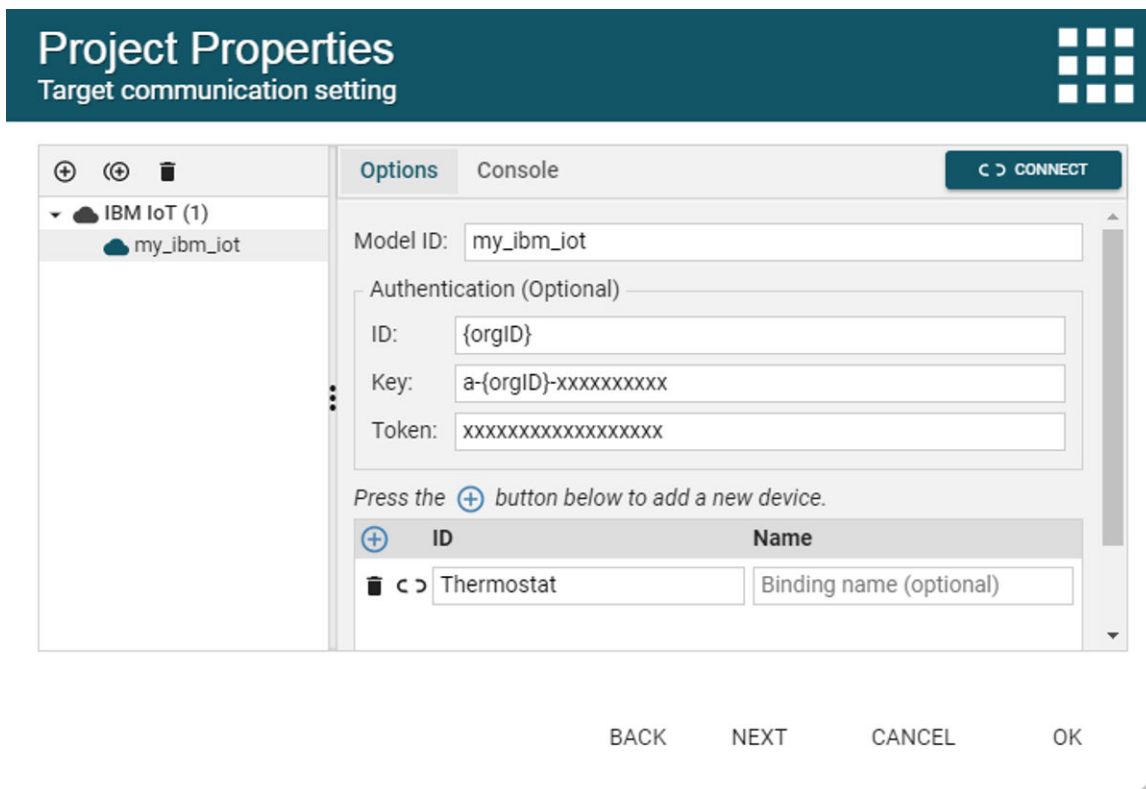
Figure 3-24. GUI Composer Project Properties
