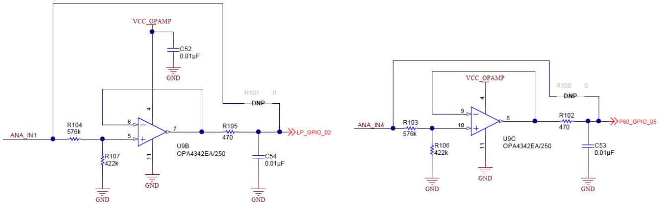
Figure 3-11. Original Circuit for ADC Buffer
