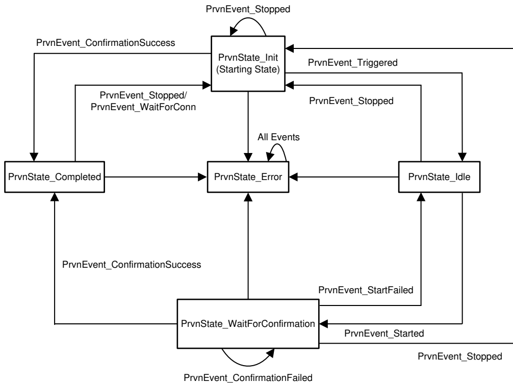
Figure 2-8. Provisioning Task State Machine
