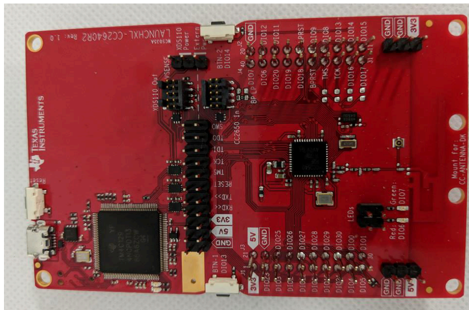
Figure 3-2. CC2640R2F LaunchPad™ Configuration
