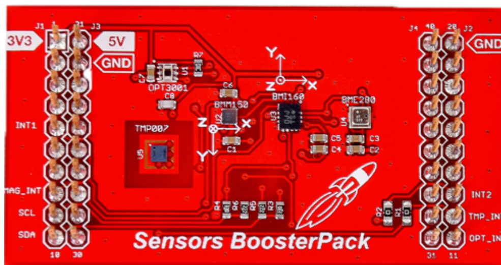
Figure 3-3. BOOSTXL-SENSORS Sensors BoosterPack™ Plug-In Module
