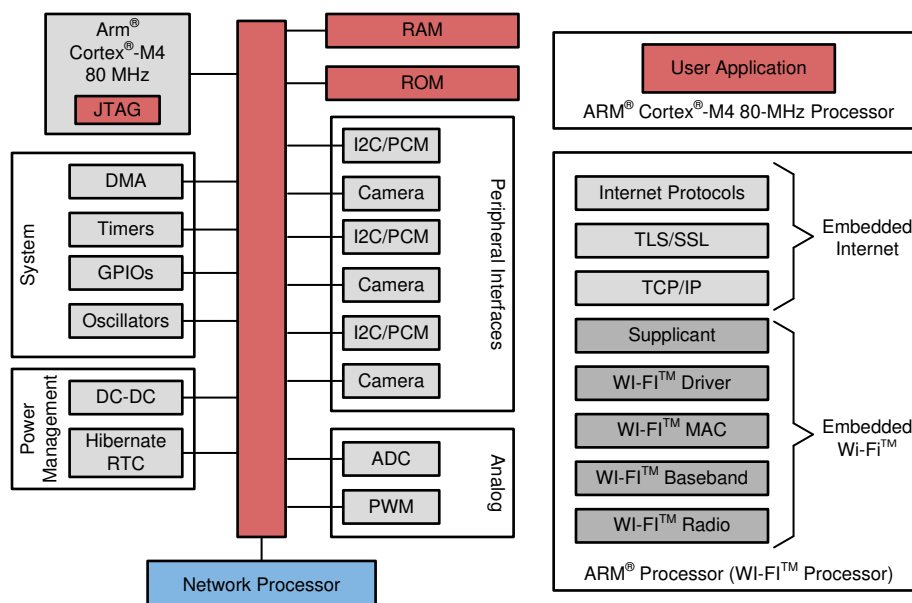
Figure 2-2. CC3220x Device Block Diagram
