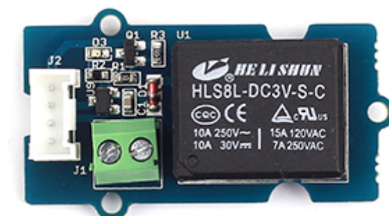
Figure 3-8. Grove – Relay
