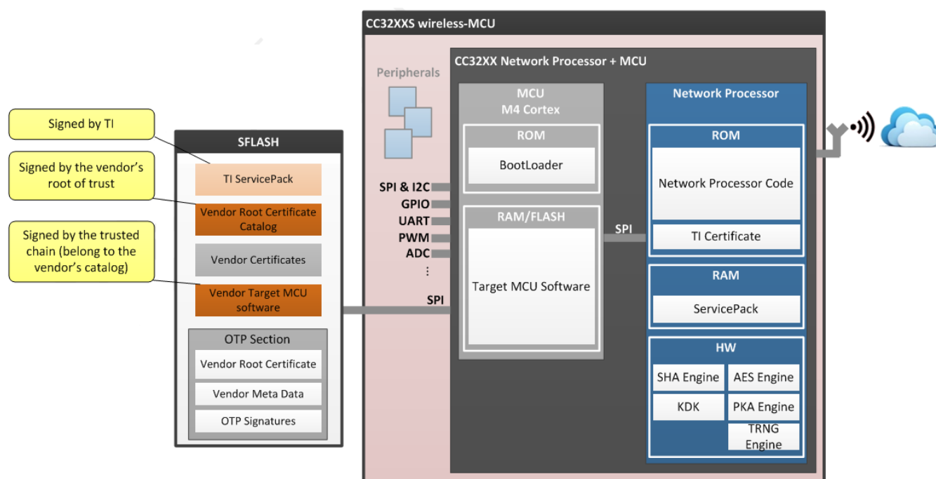
Figure 1. Architecture Scheme
