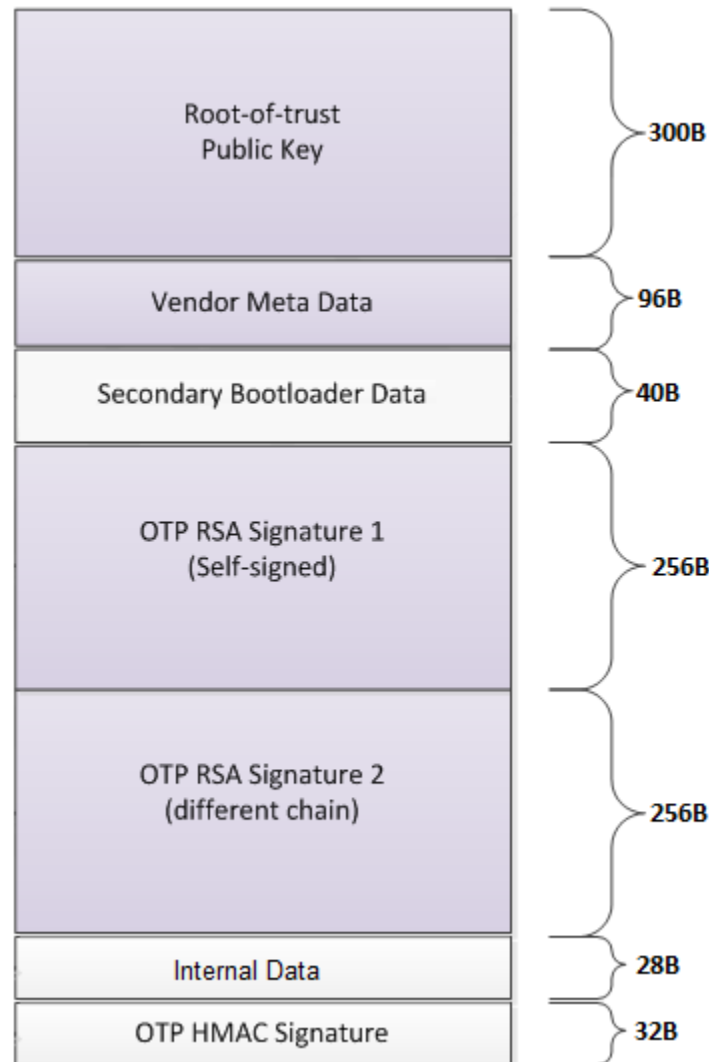
Figure 4. OTP Block
