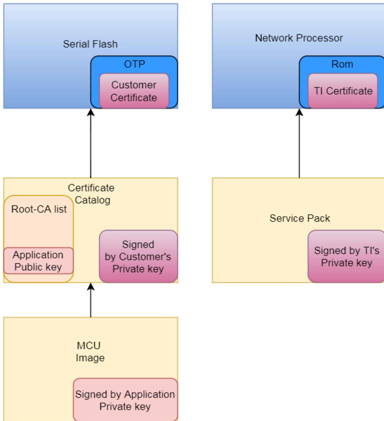
Figure 3. Customized Authentication Flow
