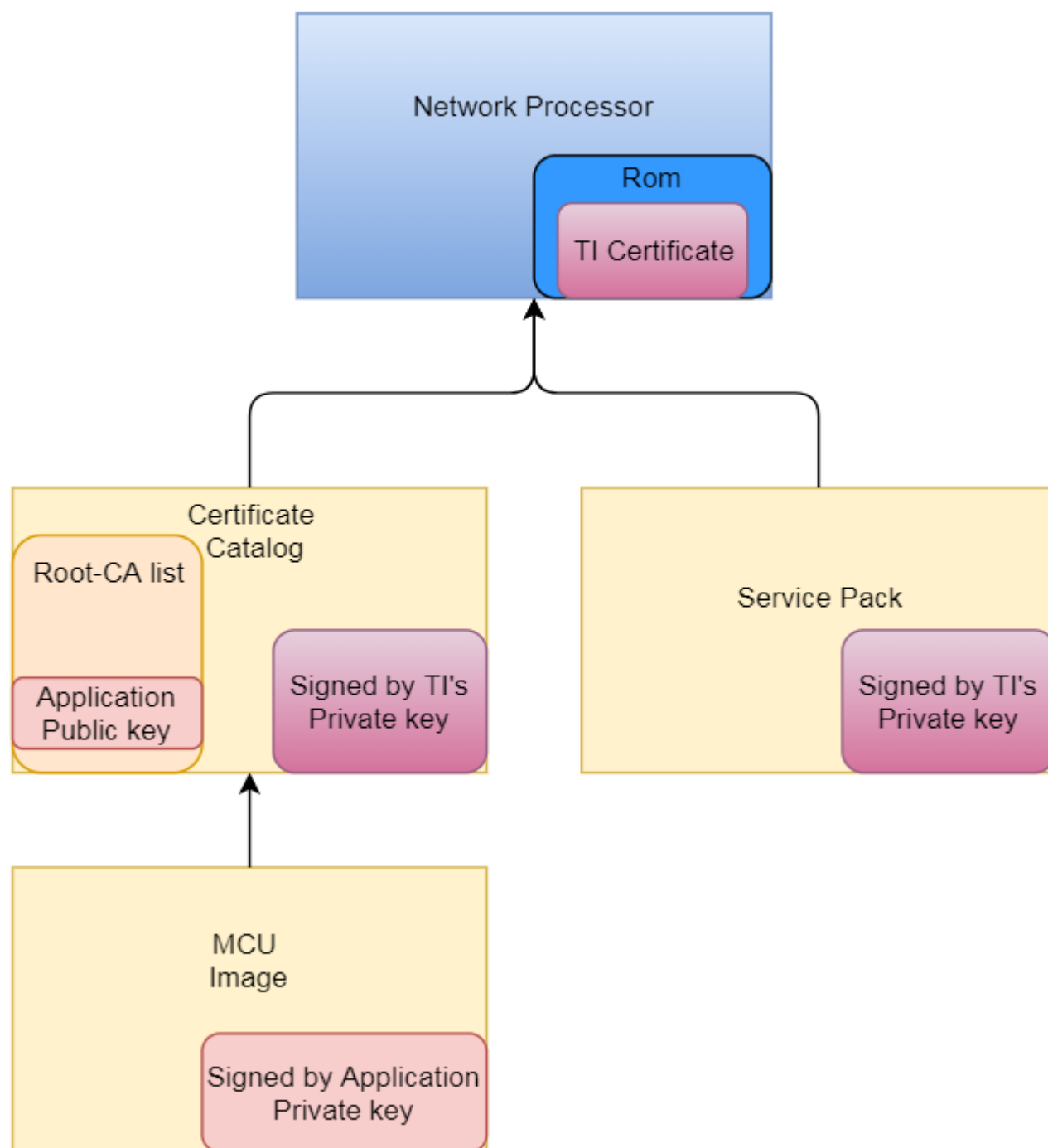
Figure 2. Basic Authentication Flow
