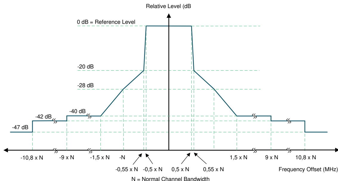
Figure 6-1. Transmit Spectral Power Mask
