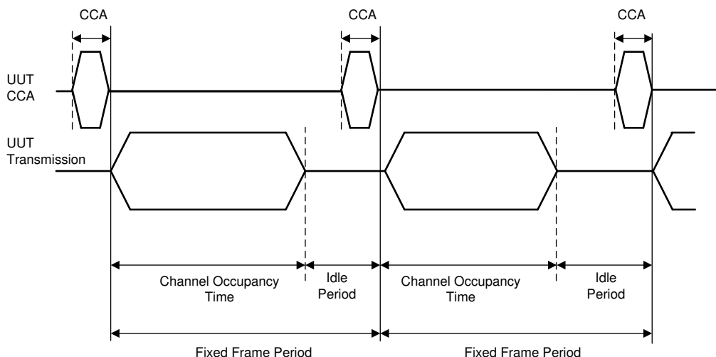
Figure 6-2. Example of timing for Frame Based Equipment
