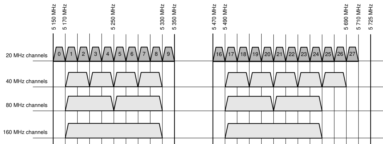
Figure 6-3. Channel Bonding for option 2
