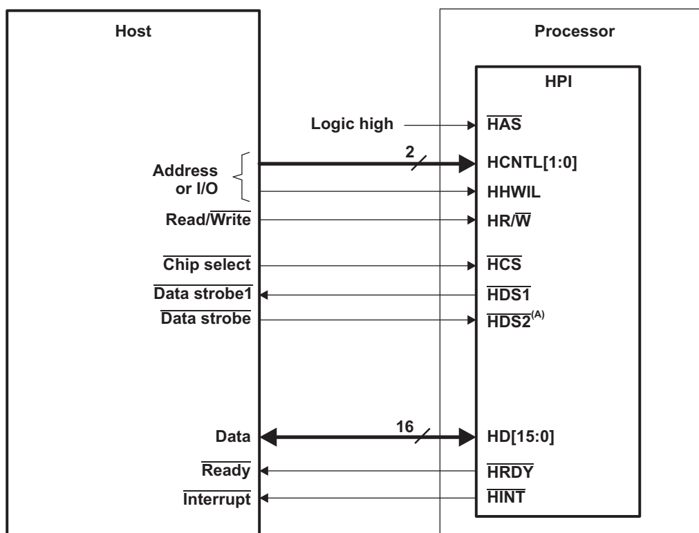
Figure 2. Example of Host-Processor Signal Connections
