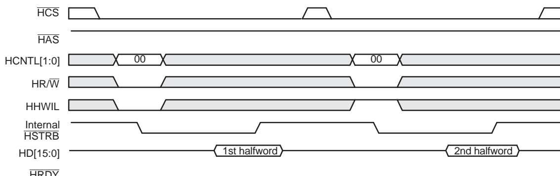
Figure 10. HRDY Behavior During an HPIC Write Cycle in the Multiplexed Mode
