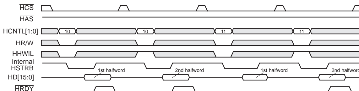
Figure 11. HRDY Behavior During a Data Write Operation in the Multiplexed Mode (Case 1: No Autoincrementing)
