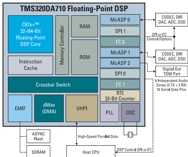
TMS320DA710 floating-point DSP block diagram
