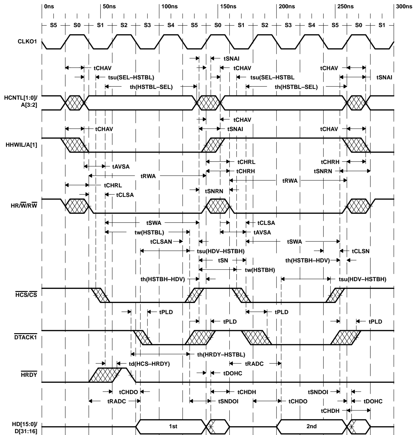
Figure 4. MC68360 Write to TMS320C62x/C67x/C64x (HPI16 Mode) HPI
