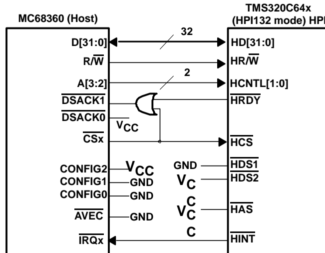
Figure 2. MC68360 to TMS320C64x (HPI32) HPI Interface Block Diagram
