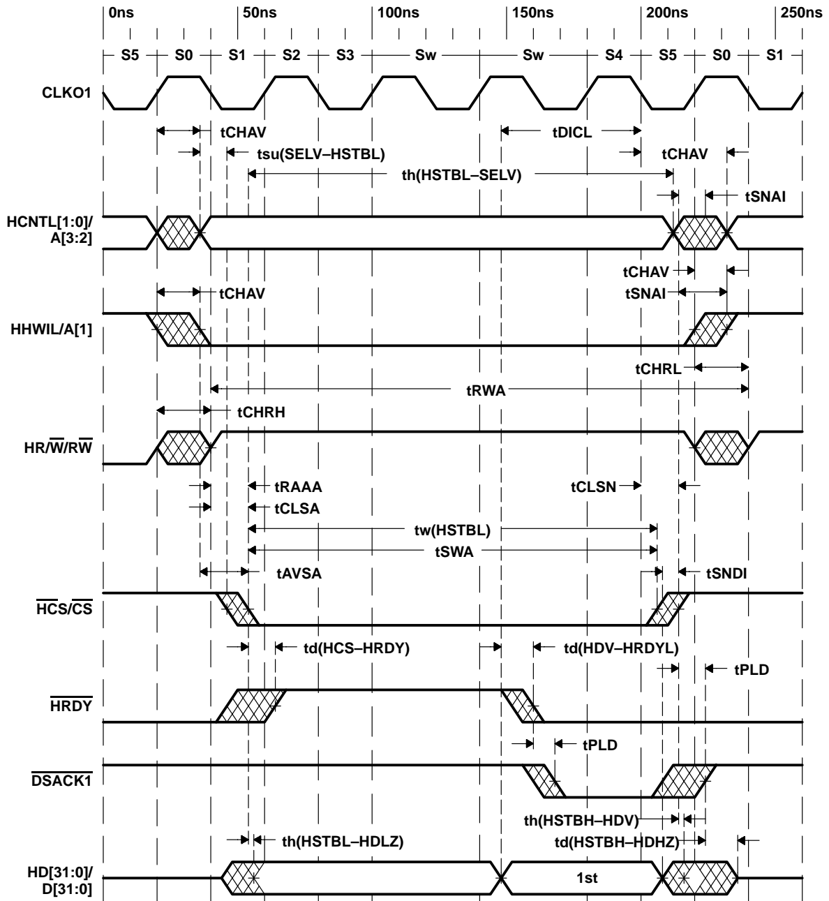
Figure 5. MC68360 Reads Internal Memory of TMS320C64x (HPI32 Mode) Using HPI (Read Without Auto-Increment)
