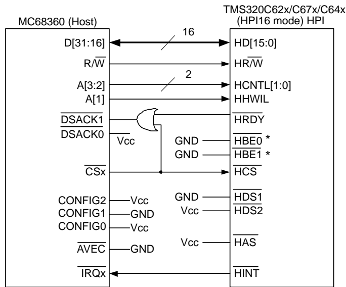
Figure 1. MC68360 to TMS320C62x/C67x/C64x (HPI16) HPI Interface Block Diagram
