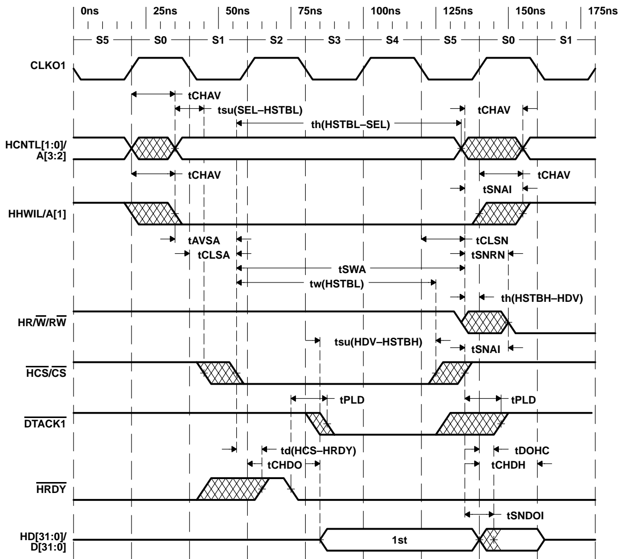
Figure 6. MC68360 Write to TMS320C64x (HPI32 Mode) HPI
