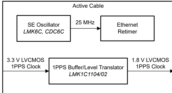
Figure 11. Example active cable clock architecture.
