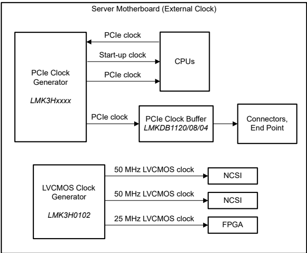
Figure 4. Example server motherboard external clock architecture.
