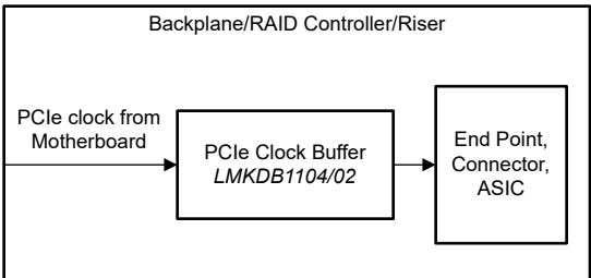
Figure 6. Example PCIe add-in cards clock architecture.
