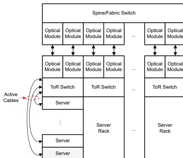
Figure 1. Data center architecture.
