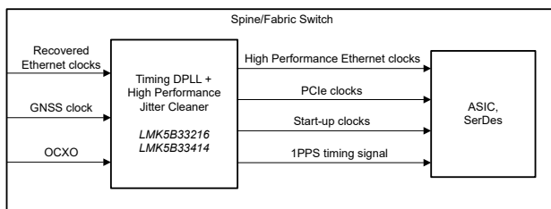
Figure 13. Simplified spine or fabric switch clock architecture.
