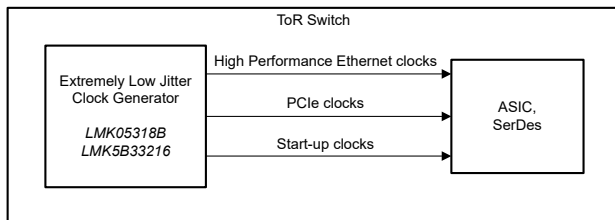
Figure 12. Simplified ToR switch clock architecture.
