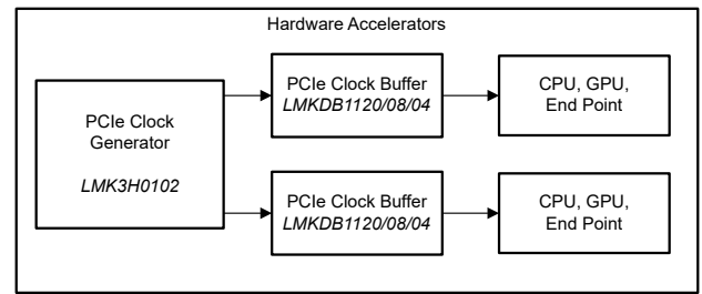
Figure 8. Example hardware accelerator clock architecture.
