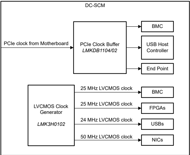
Figure 5. Example DC-SCM clock architecture.
