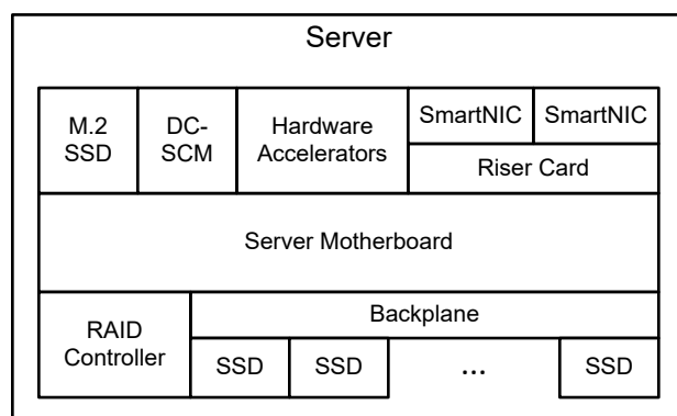
Figure 2. Server blocks.
