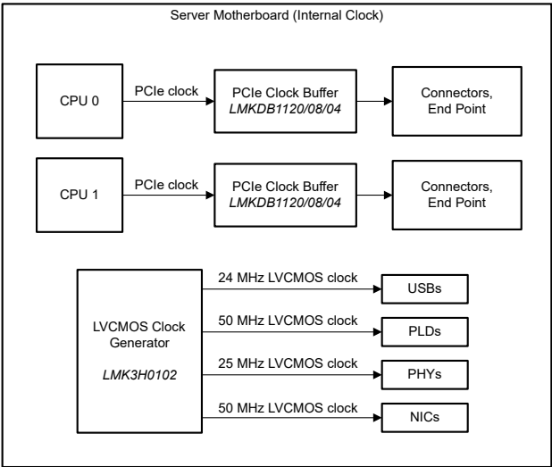
Figure 3. Example server motherboard internal clock architecture.
