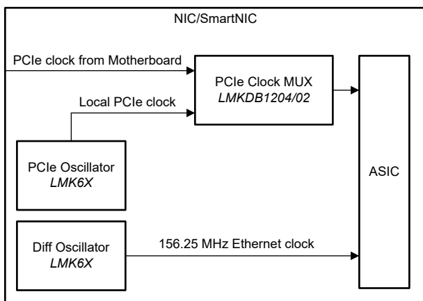
Figure 7. Example NIC and SmartNIC clock architecture.
