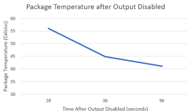
Figure 3-2. Package Temperature After Output Disabled
