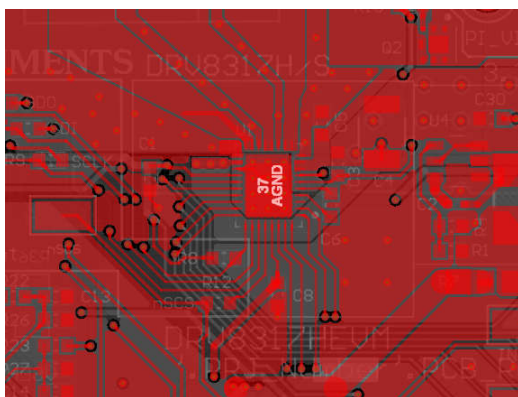
Figure 3-3. DRV8317HEVM Layout
