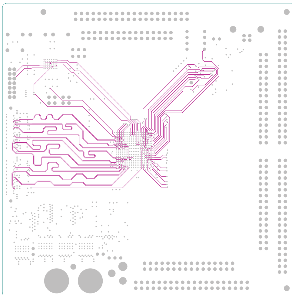
Figure 22. TSW1200C Layout Layer 5
