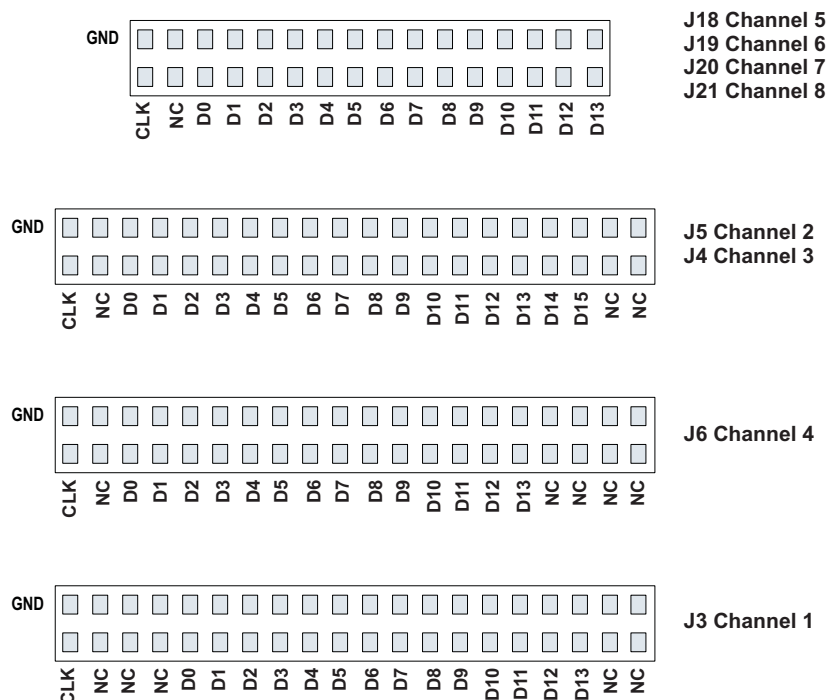
Figure 6. Pinout of Header Posts for Parallel Output Data
