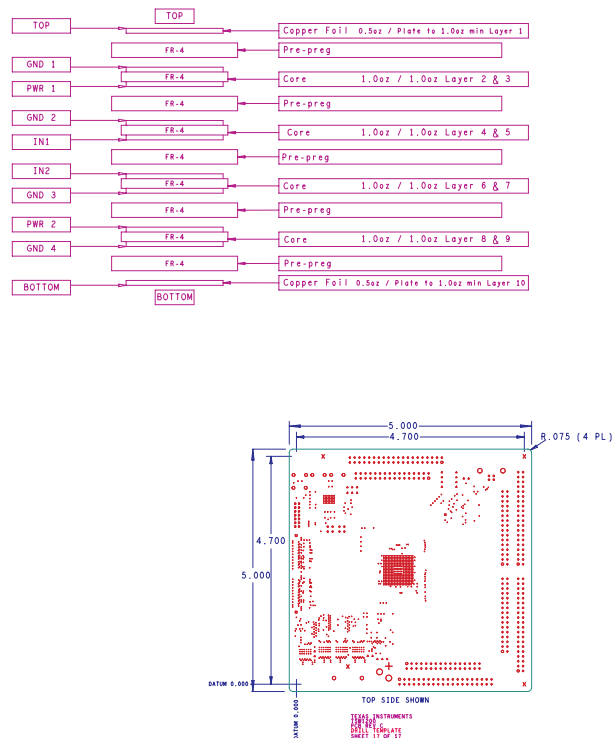
Figure 25. Circuit Board Stackup
