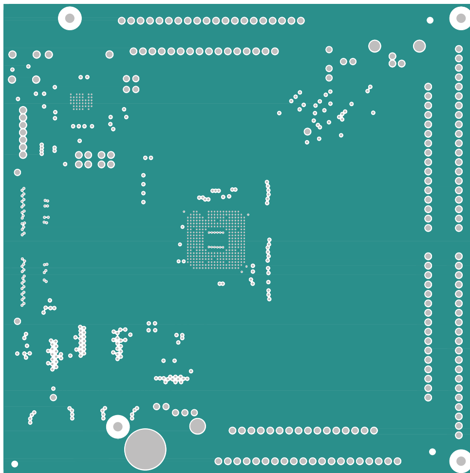
Figure 21. TSW1200C Layout Ground Plane
