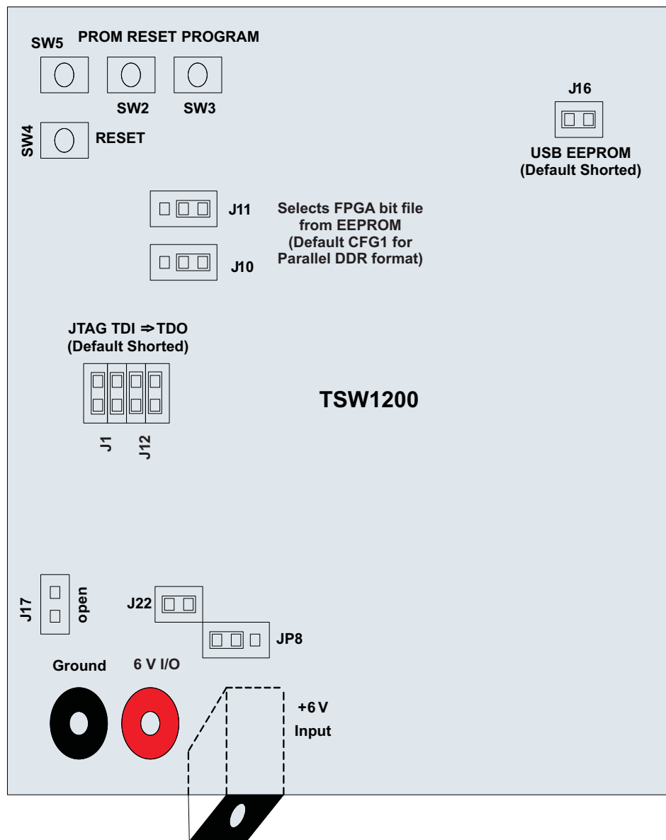
Figure 2. Position of Switches and Jumpers
