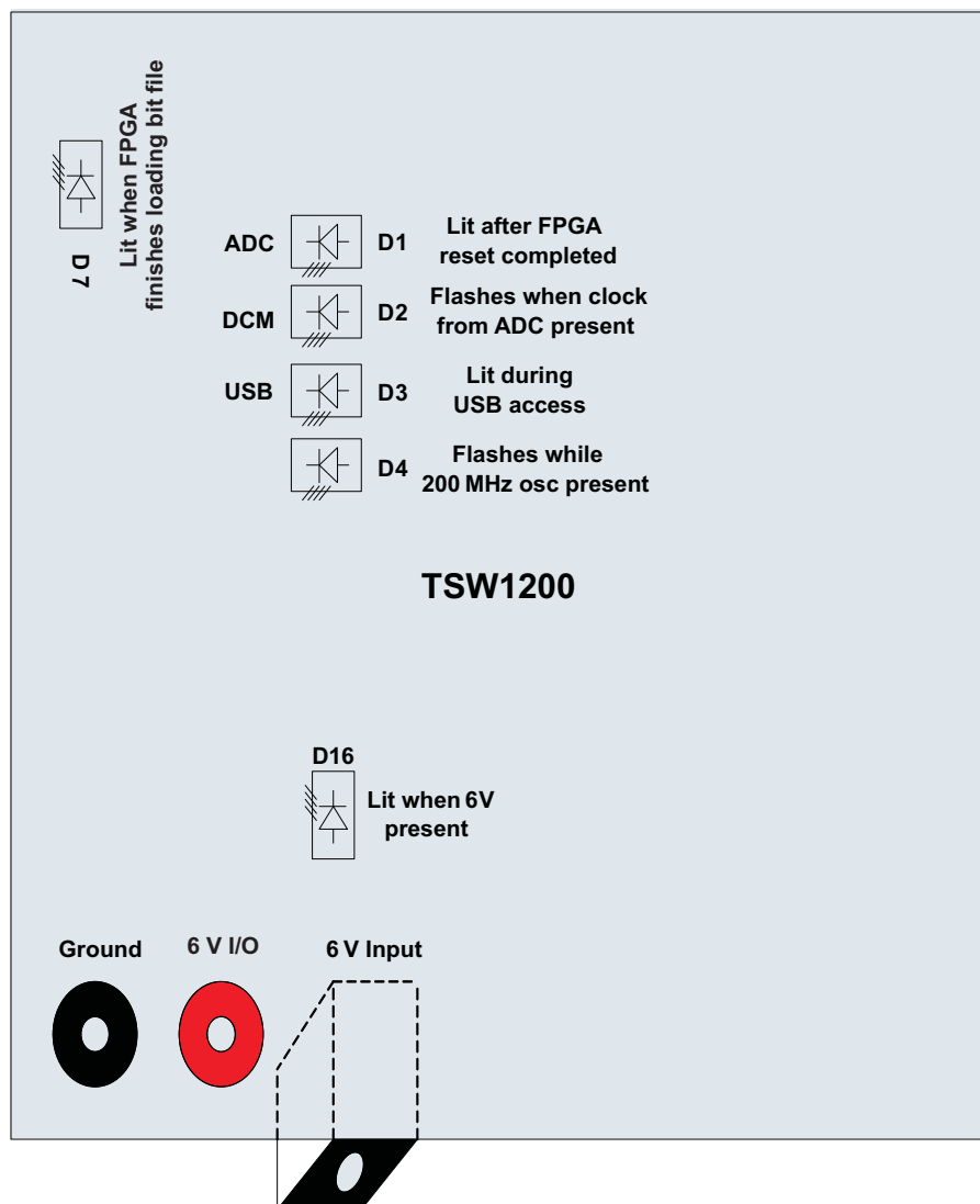
Figure 4. Position of LEDs
