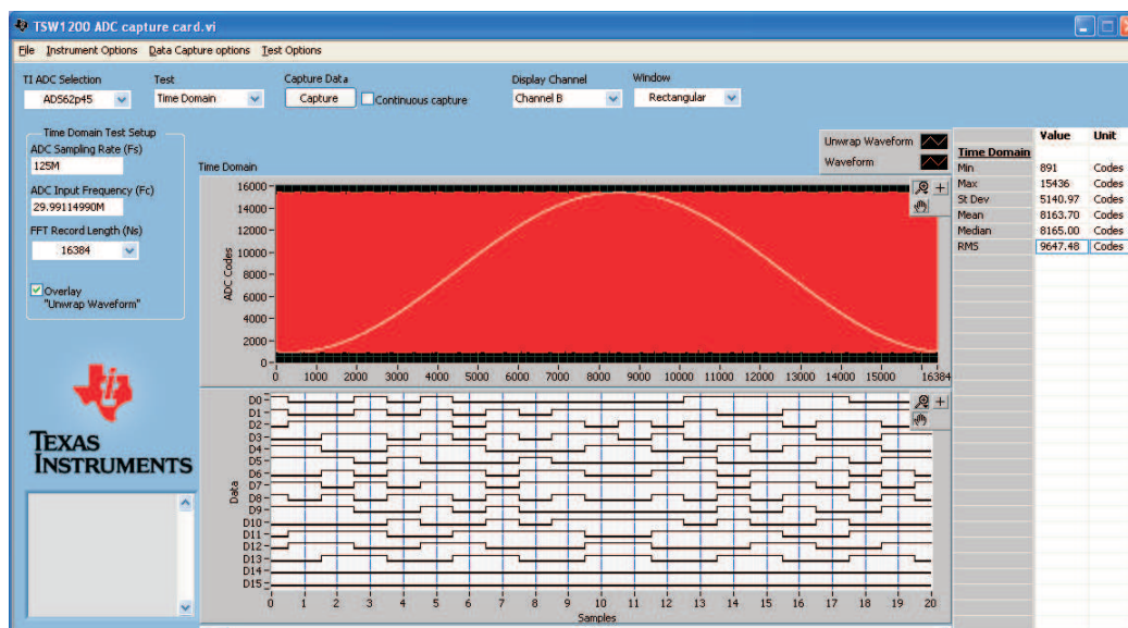
Figure 12. User Interface Time Domain Format
