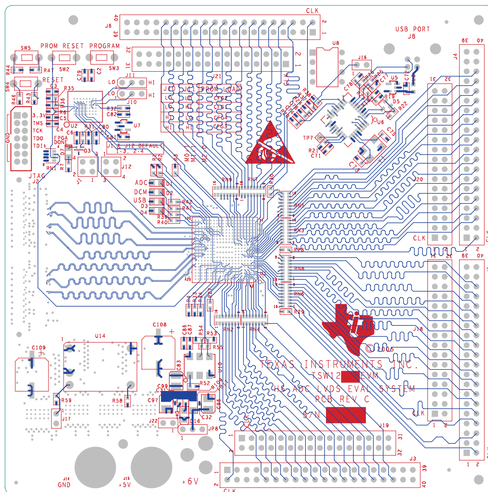
Figure 19. TSW1200C Layout Layer Two
