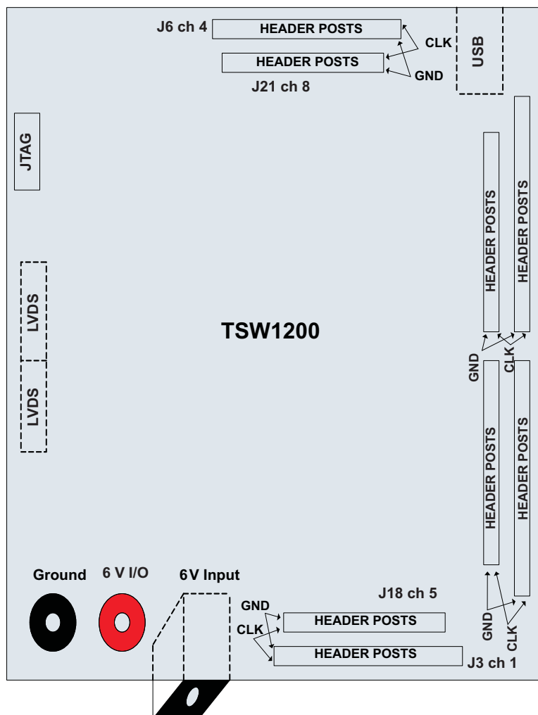
Figure 5. Position of Input, Output, and USB Connections
