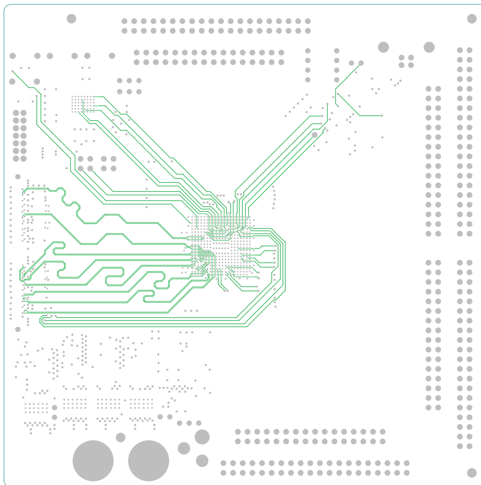
Figure 23. TSW1200C Layer 6
