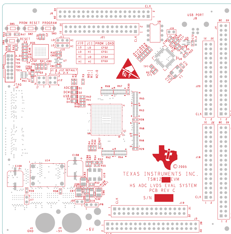
Figure 18. TSW1200C Layout Top Layer
