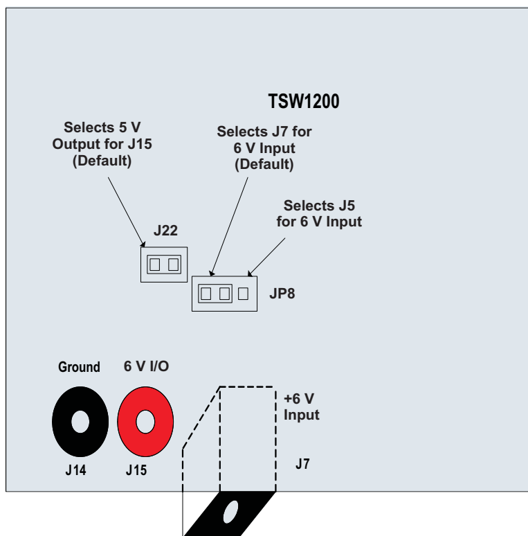
Figure 1. Position of Power Connections
