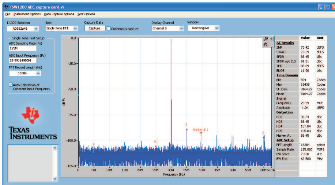
Figure 11. User Interface Single FFT format
