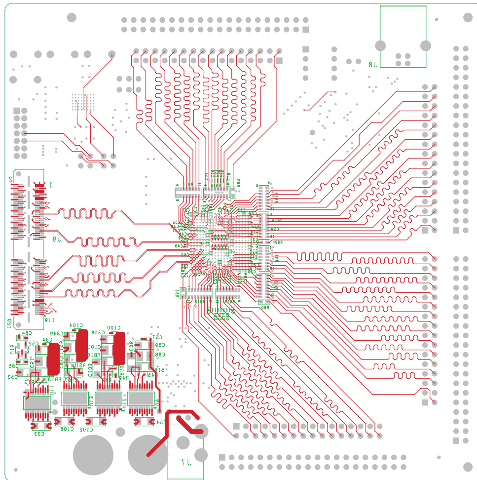
Figure 24. TSW1200C Bottom Layer
