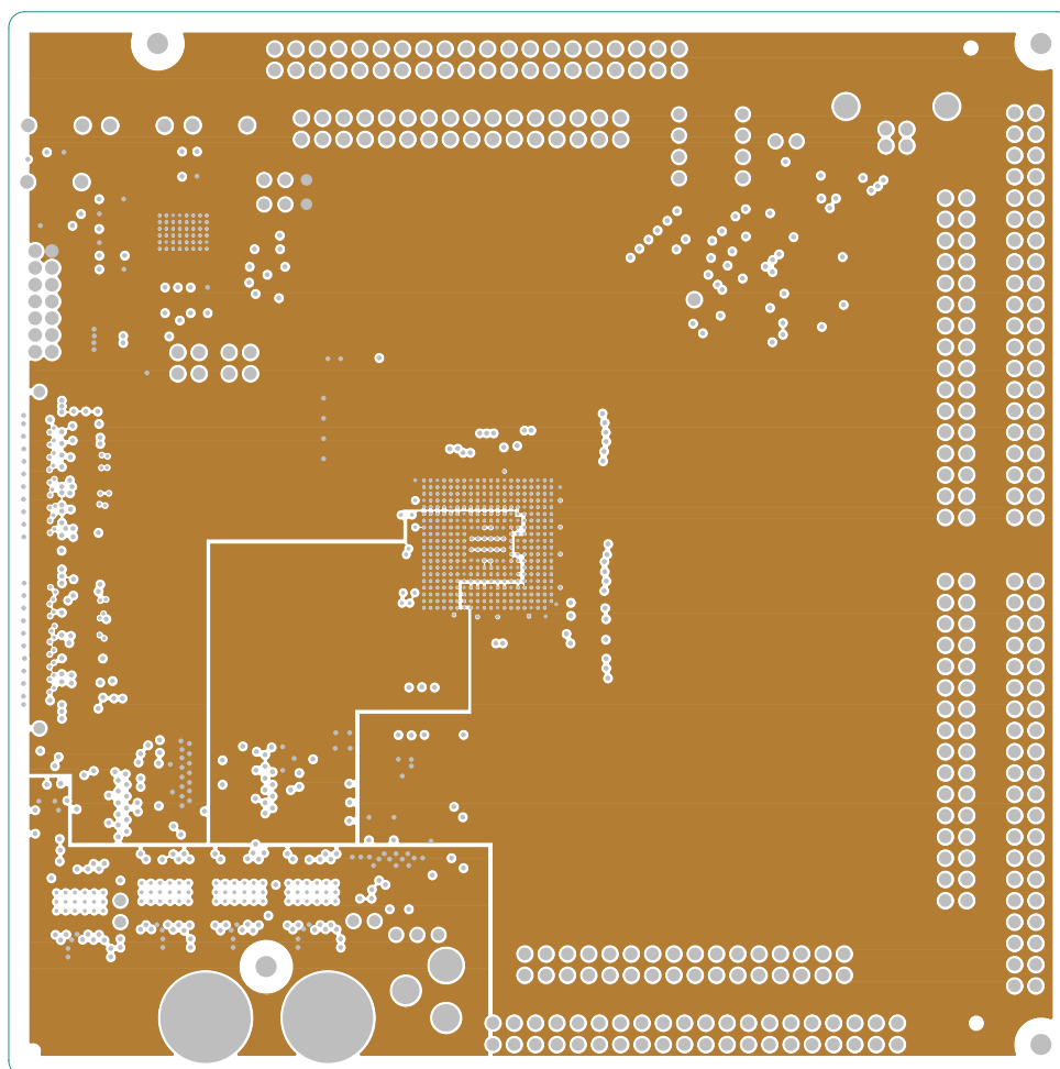
Figure 20. TSW1200C Layout Power Plane
