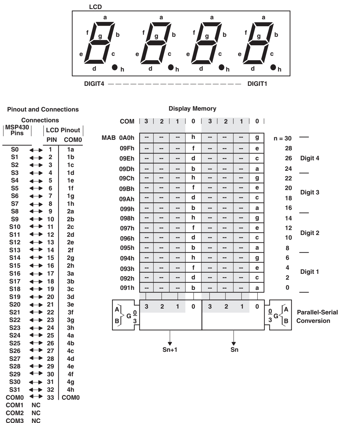
Figure 34-5. Static LCD Example (MAB addresses need to be replaced with LCDMx)
