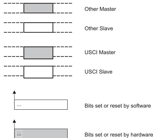
Figure 41-8. I 2 C Time-Line Legend
