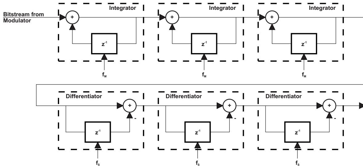
Figure 29-6. SINC 3 Filter Structure
