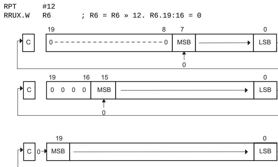
Figure 6-54. Rotate Right Unsigned RRUX(.B,.A) – Register Mode
