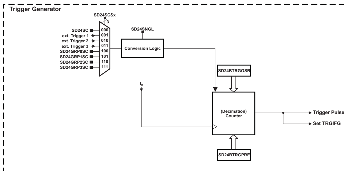
Figure 29-15. SD24_B Trigger Generator Block Diagram
