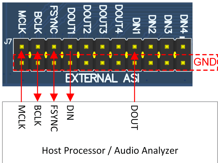
Figure 4-5. AC-MB Connection with External Audio Serial Interface
