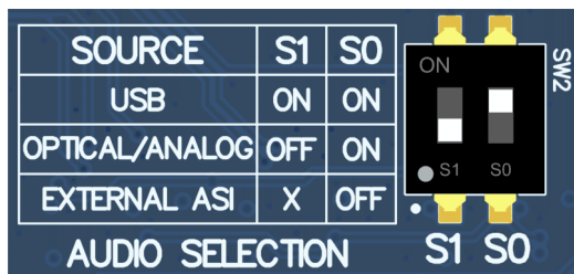
Figure 4-3. AC-MB Optical or Auxiliary Analog Audio Setting
