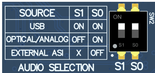
Figure 4-2. AC-MB USB Audio Setting
