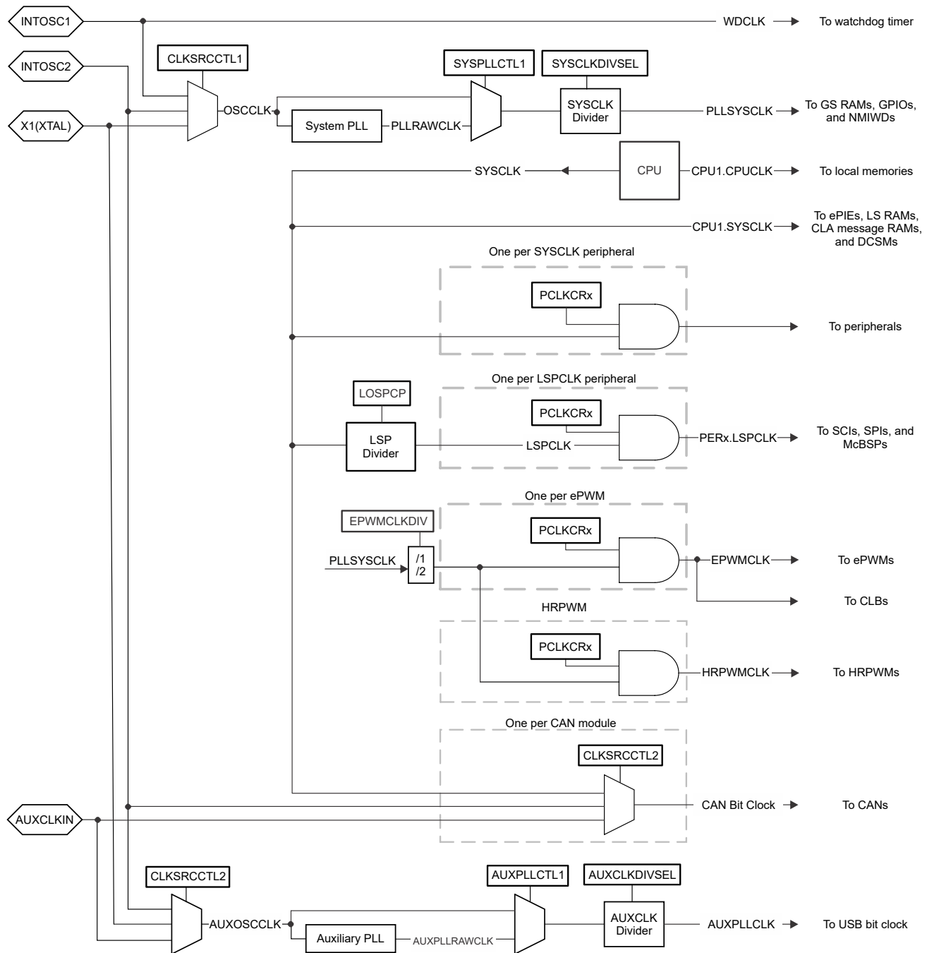
Figure 6-7. Clocking System
