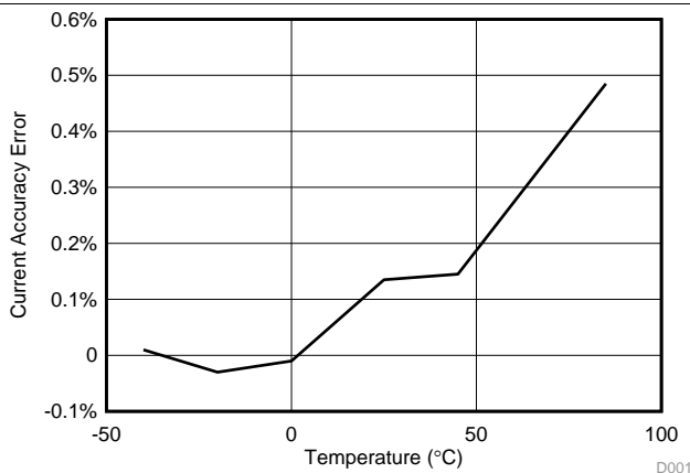
Figure 3. Current Accuracy Error vs. Temperature D001
