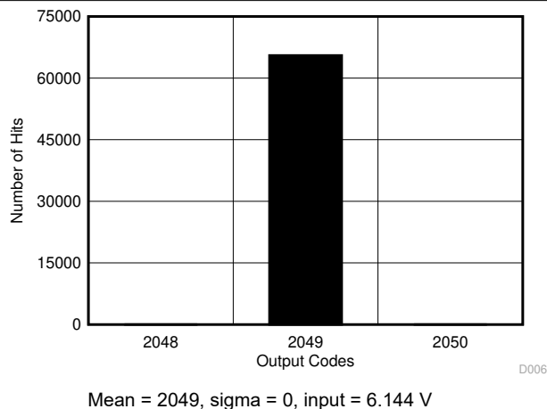
Figure 6-18. DC Histogram for Mid-Scale Inputs ( 0\text{ V} – 12.288\text{ V} )
