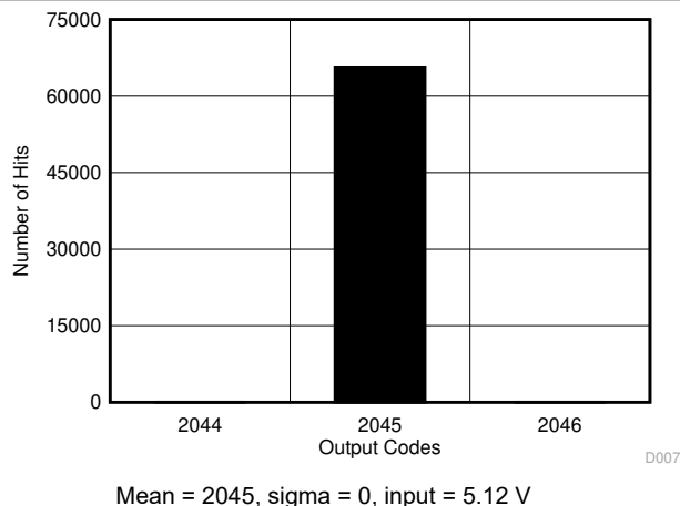
Figure 6-19. DC Histogram for Mid-Scale Inputs ( 0\text{ V} – 10.24\text{ V} )
