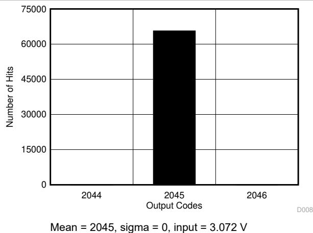
Figure 6-20. DC Histogram for Mid-Scale Inputs ( 0\text{ V} – 6.144\text{ V} )
