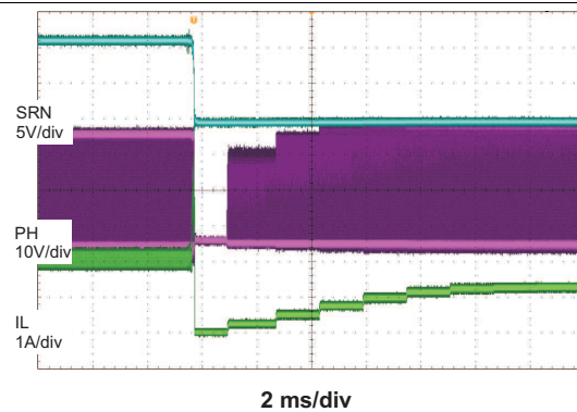
Figure 8. System Load Transient (Input Current DPM)
