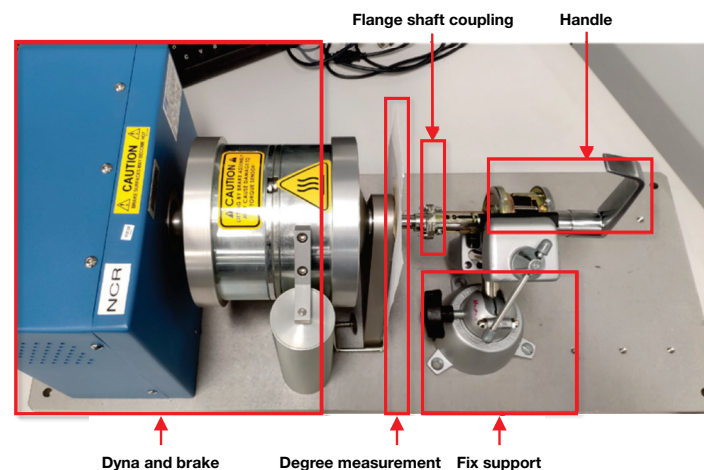
Figure 6. Door handle energy harvesting test setup.
