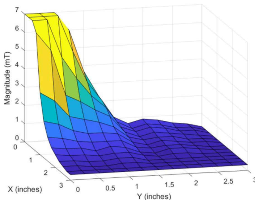
Figure 7-6. TMAG5170 Off-Axis Magnetic Detection
