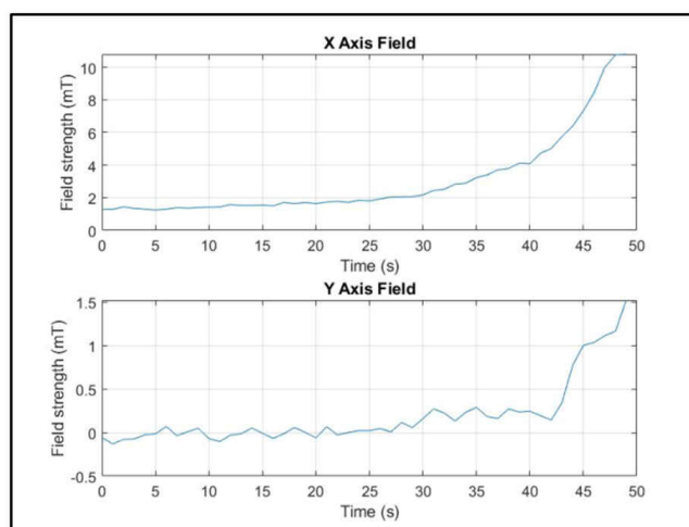
Figure 7-8. TMAG5170 Orthogonal-Axis Magnetic Detection: Results
