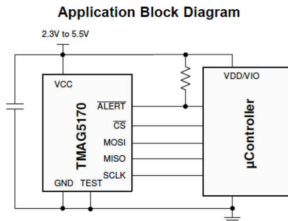
Figure 3-3. Application Block Diagram
