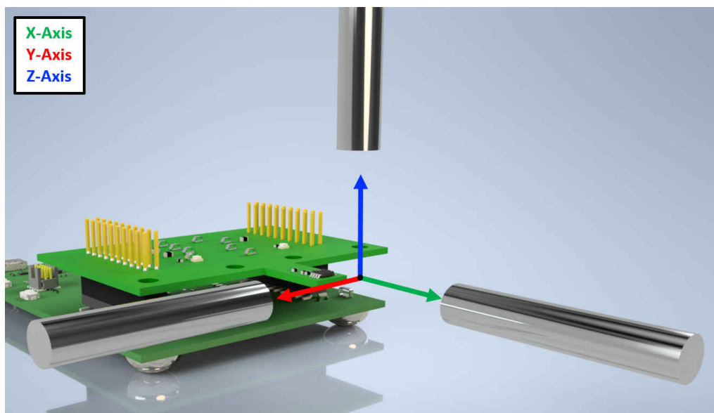
Figure 7-2. TMA5170 Magnetic Approach Directions
