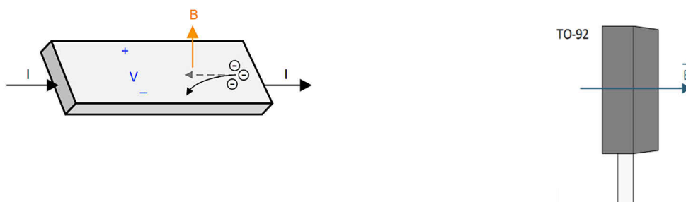
Figure 3-1. Hall Effect Sensor Working Principles and Magnetic Flux Direction
