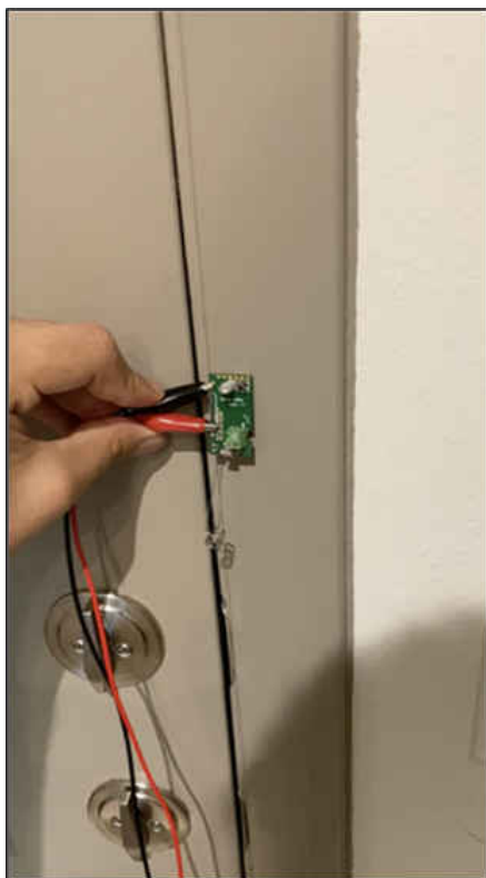
Figure 6-7. Reed Switch Tamper Susceptibility Testing Setup
