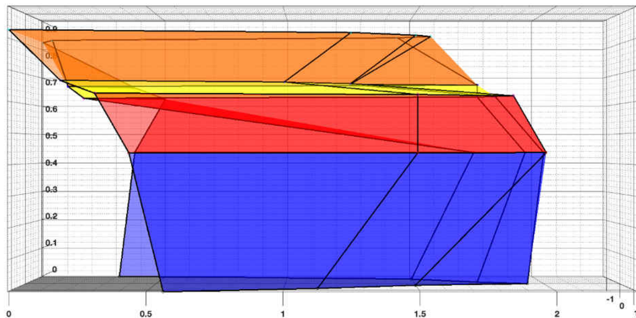
Figure 6-2. Reed Switch Front Approach Magnetic Detection Field Results: Side View
