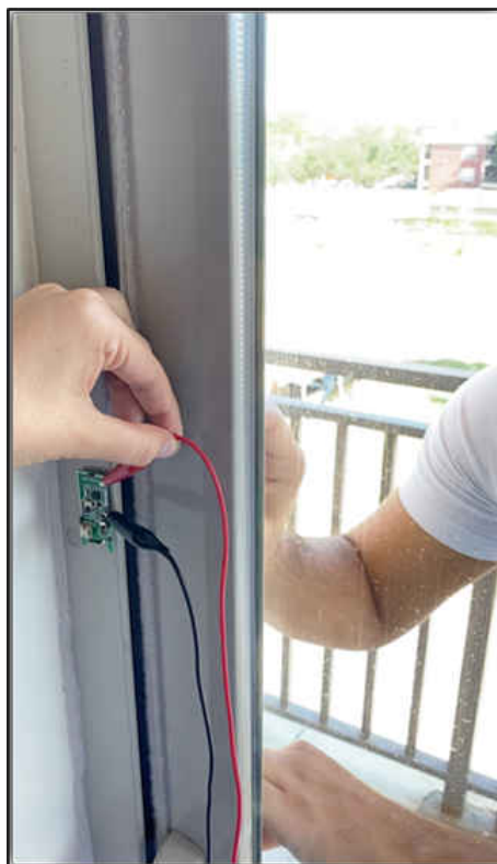
Figure 6-7. Reed Switch Tamper Susceptibility Testing Setup
