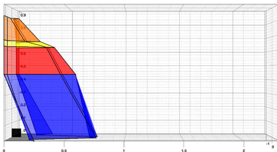
Figure 5-8. DRV5032 Side Approach Magnetic Detection Field Results: Side View
