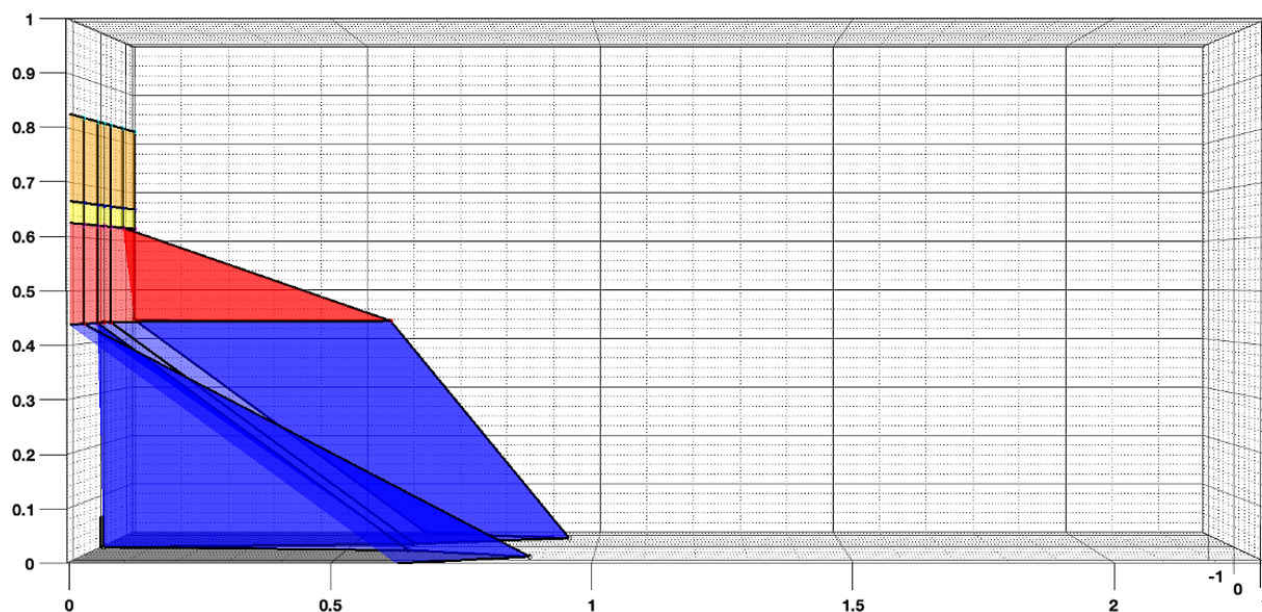
Figure 5-5. DRV5032 Front Approach Magnetic Detection Field: Side View
