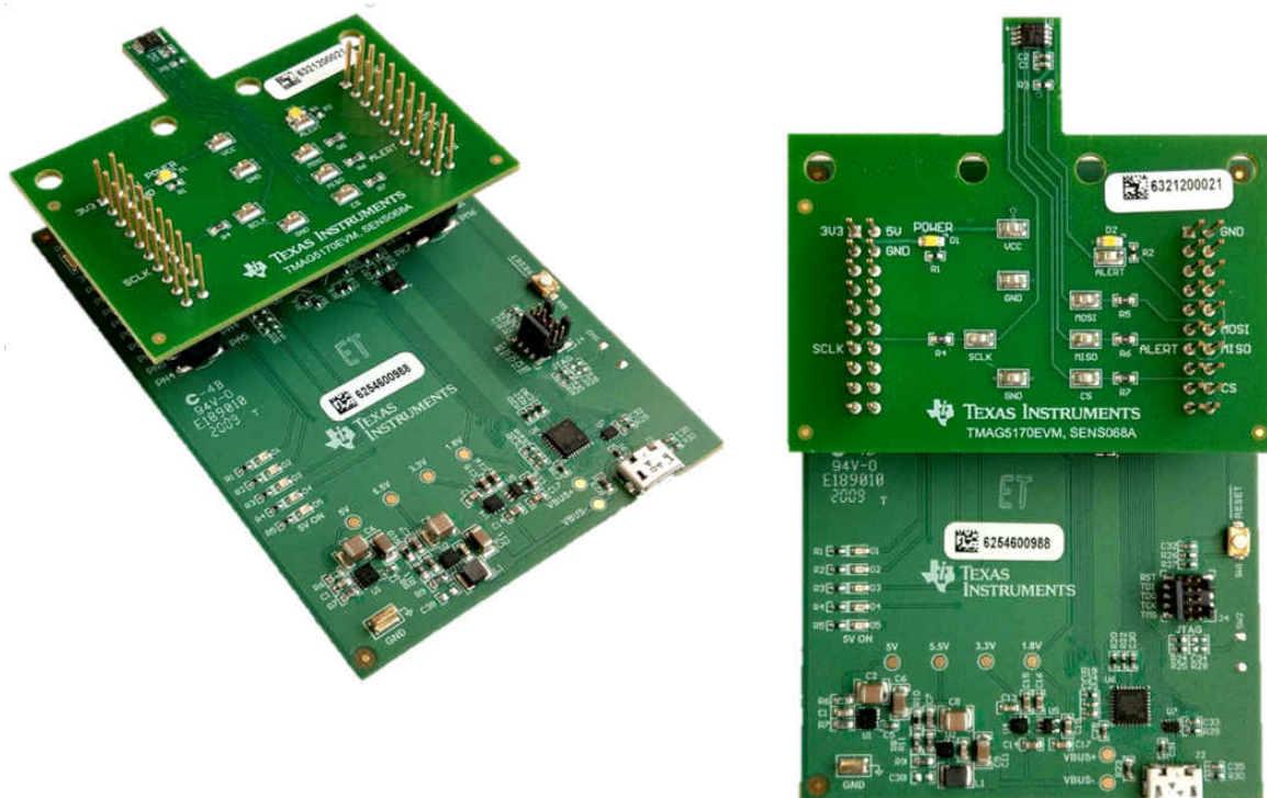
Figure 7-1. TMAG5170EVM Board
