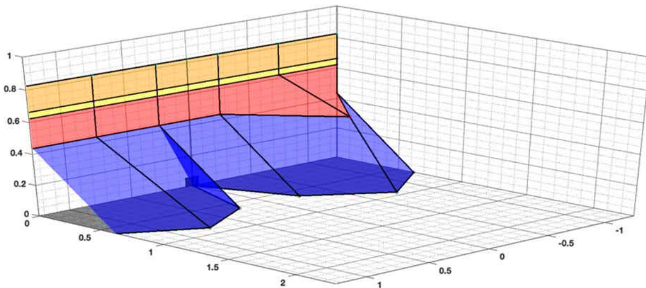
Figure 5-6. DRV5032 Front Approach Magnetic Detection Field: Off-Axis View
