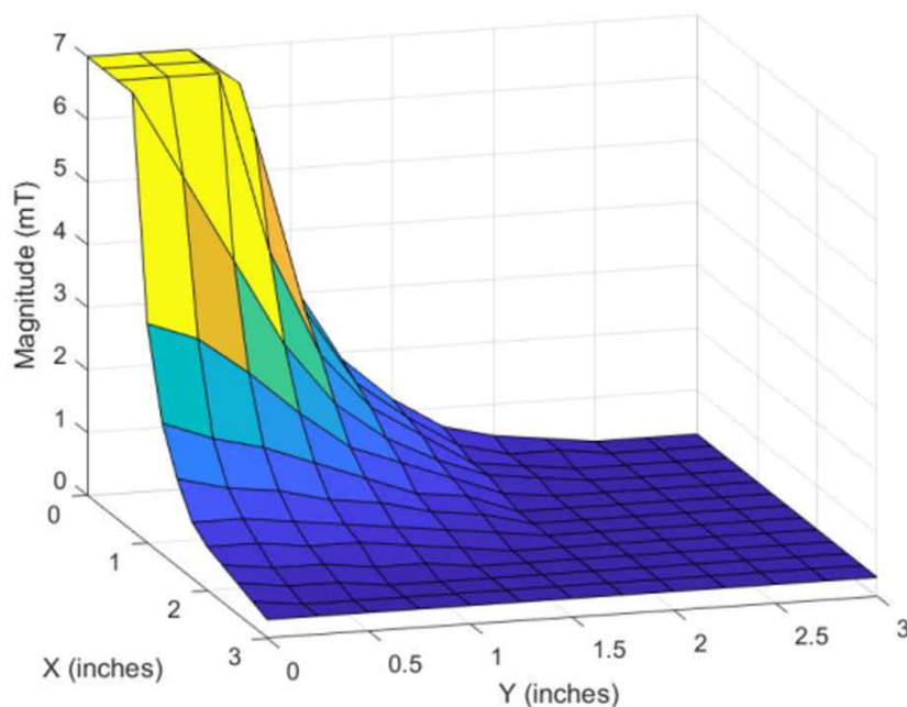
Figure 7-5. TMAG5170 On-Axis Magnetic Detection
