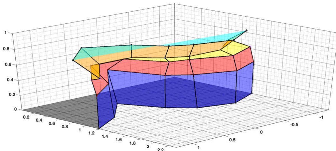
Figure 6-6. Reed Switch Side Approach Magnetic Detection Field Results: Off-Axis View
