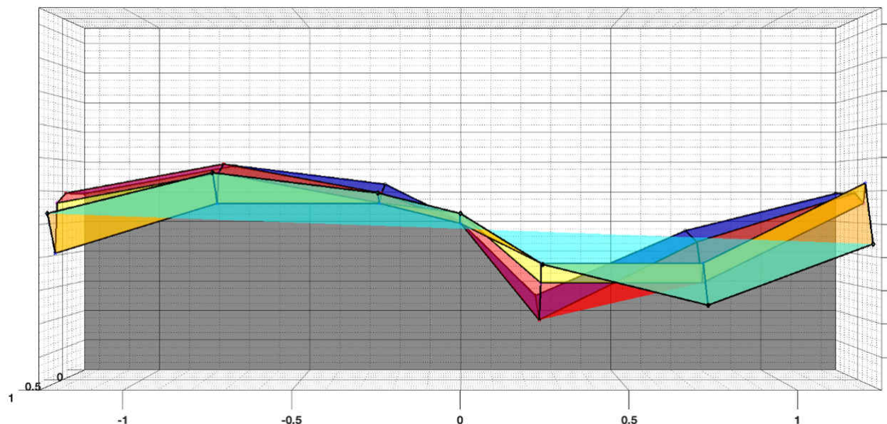
Figure 6-4. Reed Switch Side Approach Magnetic Detection Field Results: Top-down View
