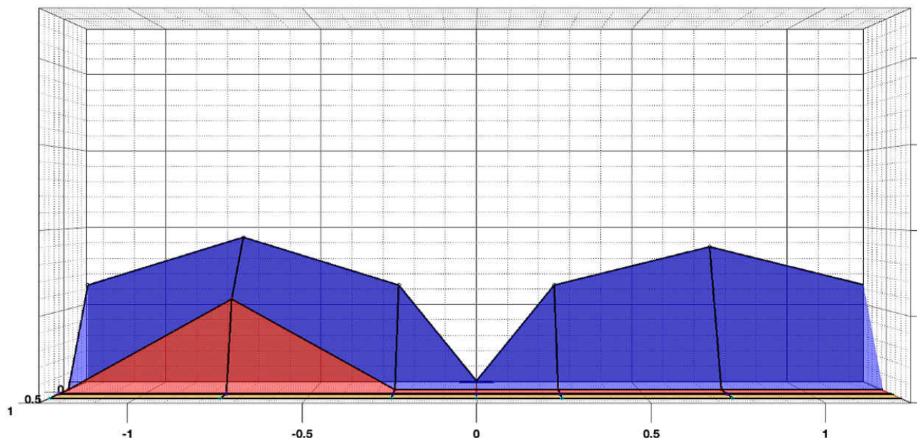
Figure 5-4. DRV5032 Front Approach Magnetic Detection Field: Top Down View
