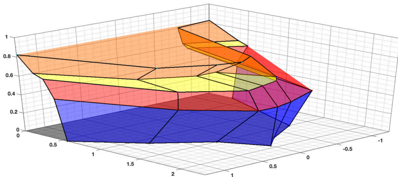
Figure 6-3. Reed Switch Front Approach Magnetic Detection Field Results: Off-Axis View
