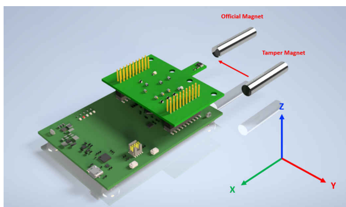
Figure 7-7. TMAG5170 Orthogonal Tamper Testing Setup
