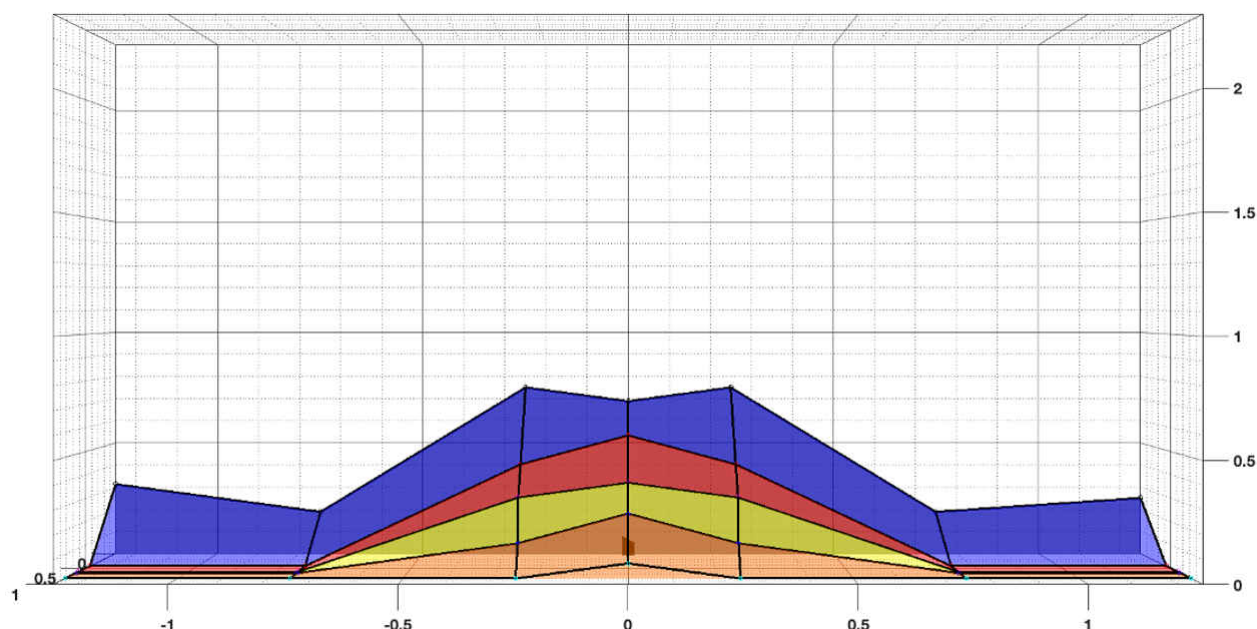
Figure 5-7. DRV5032 Side Approach Magnetic Detection Field Results: Top Down View
