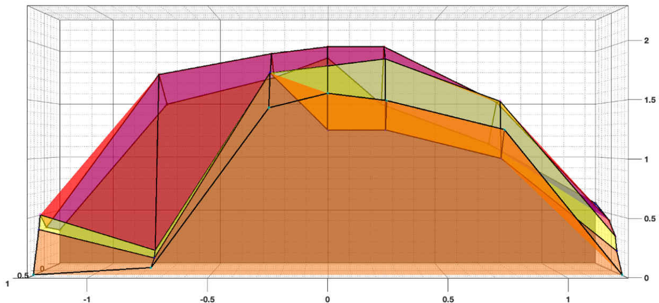
Figure 6-1. Reed Switch Front Approach Magnetic Detection Field Results: Top Down View
