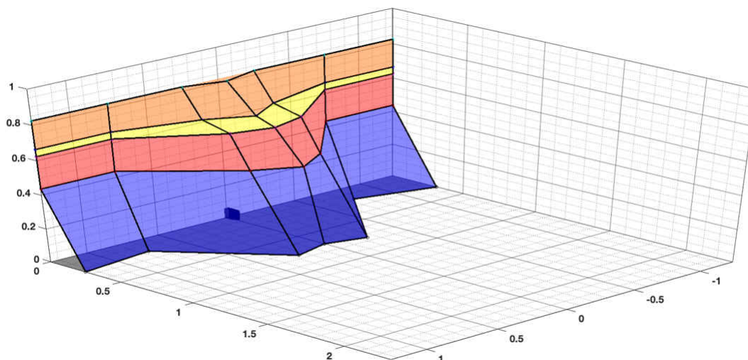
Figure 5-9. DRV5032 Side Approach Magnetic Detection Field Results: Off-Axis View
