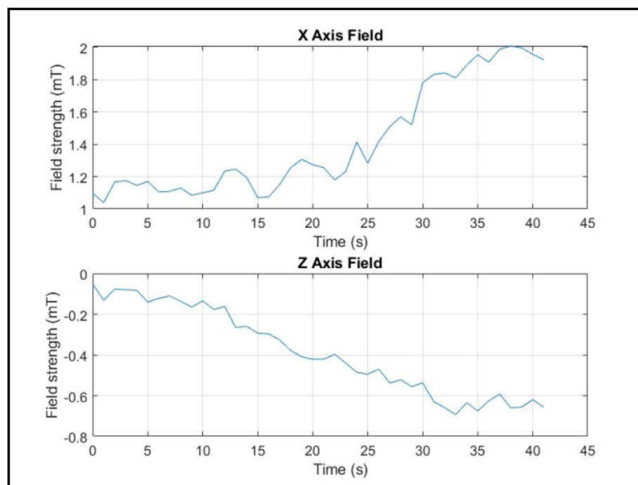
Figure 7-10. TMAG5170 Parallel Tamper Test: Results
