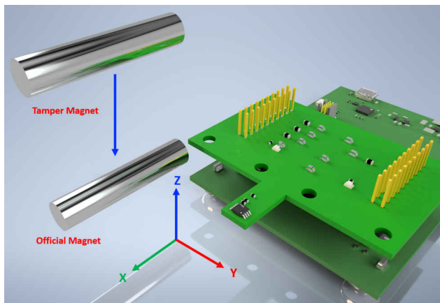
Figure 7-9. TMAG5170 Parallel Tamper Test: Setup
