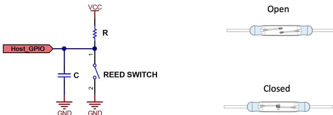
Figure 2-1. Reed Switch and Simple Circuit
