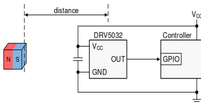
Figure 3-2. DRV5032 Application Example
