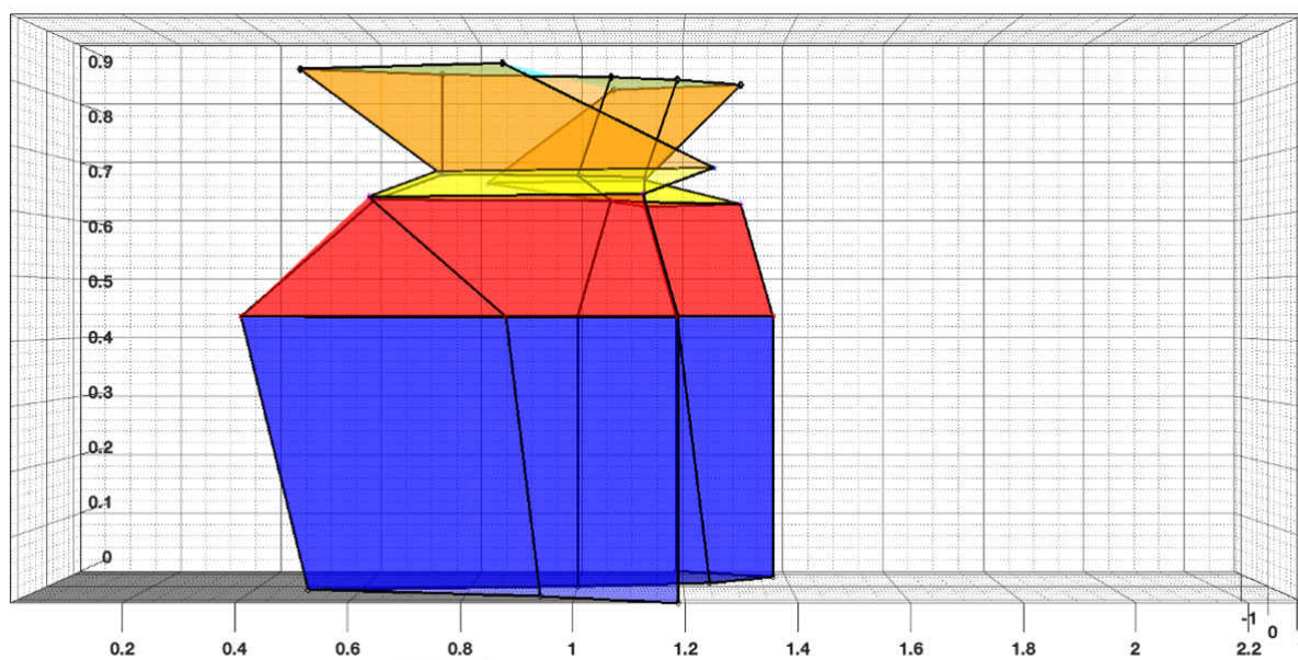
Figure 6-5. Reed Switch Side Approach Magnetic Detection Field Results: Side View
