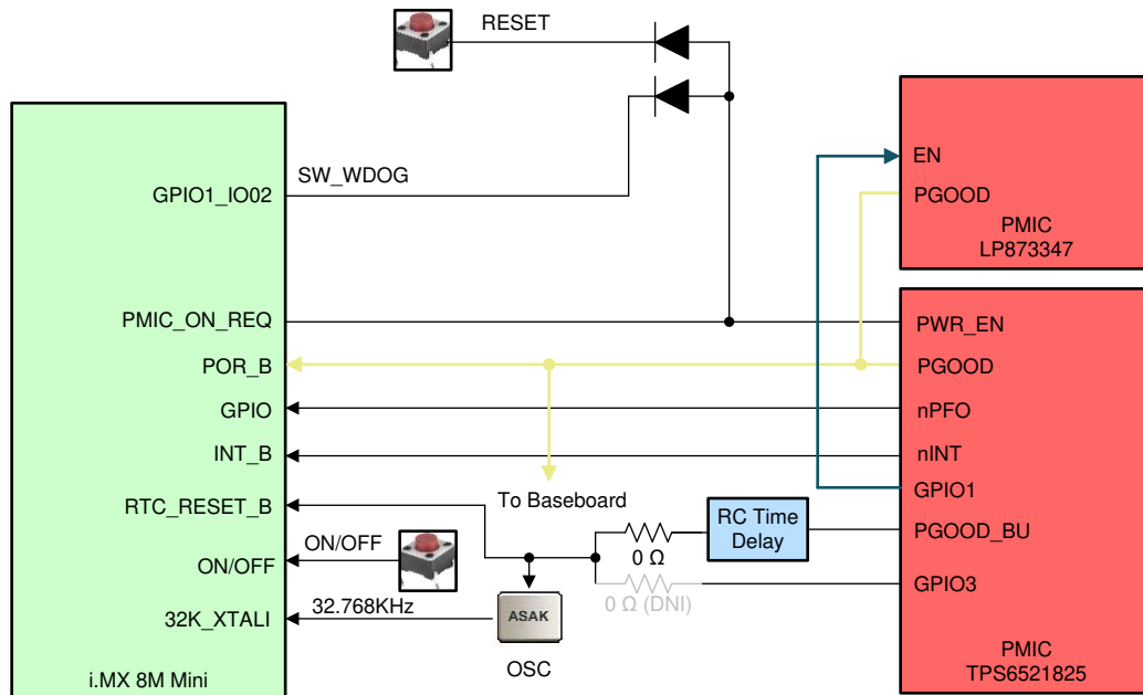
Figure 10. Reset Scheme
