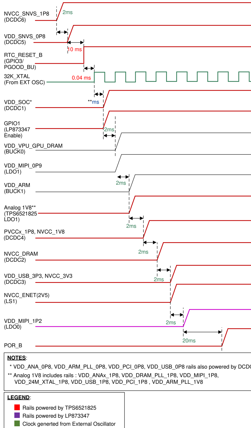
Figure 9. Required Power Sequence for i.MX 8M Mini Processor
