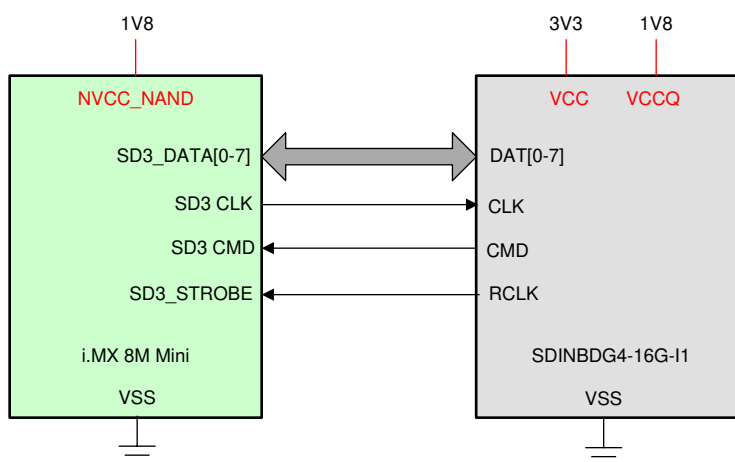
Figure 3. eMMC interface
