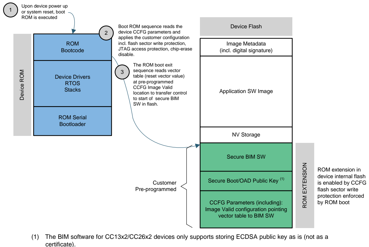
Figure 4. Hardware RoT for Secure Boot
