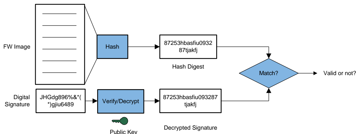
Figure 2. Verifying Digital Signature of the Firmware
