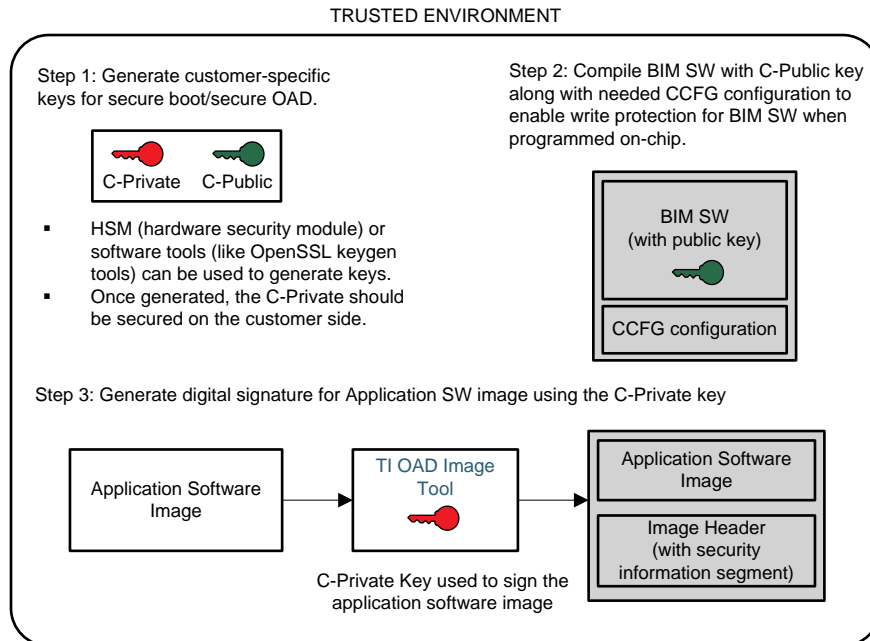
Figure 5. Initial Programming Flow With TI Provided Tools to Facilitate Secure Boot on SimpleLink CC13x2/CC26x2 Devices
