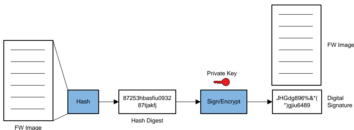
Figure 1. Generating Digital Signature of the Firmware
