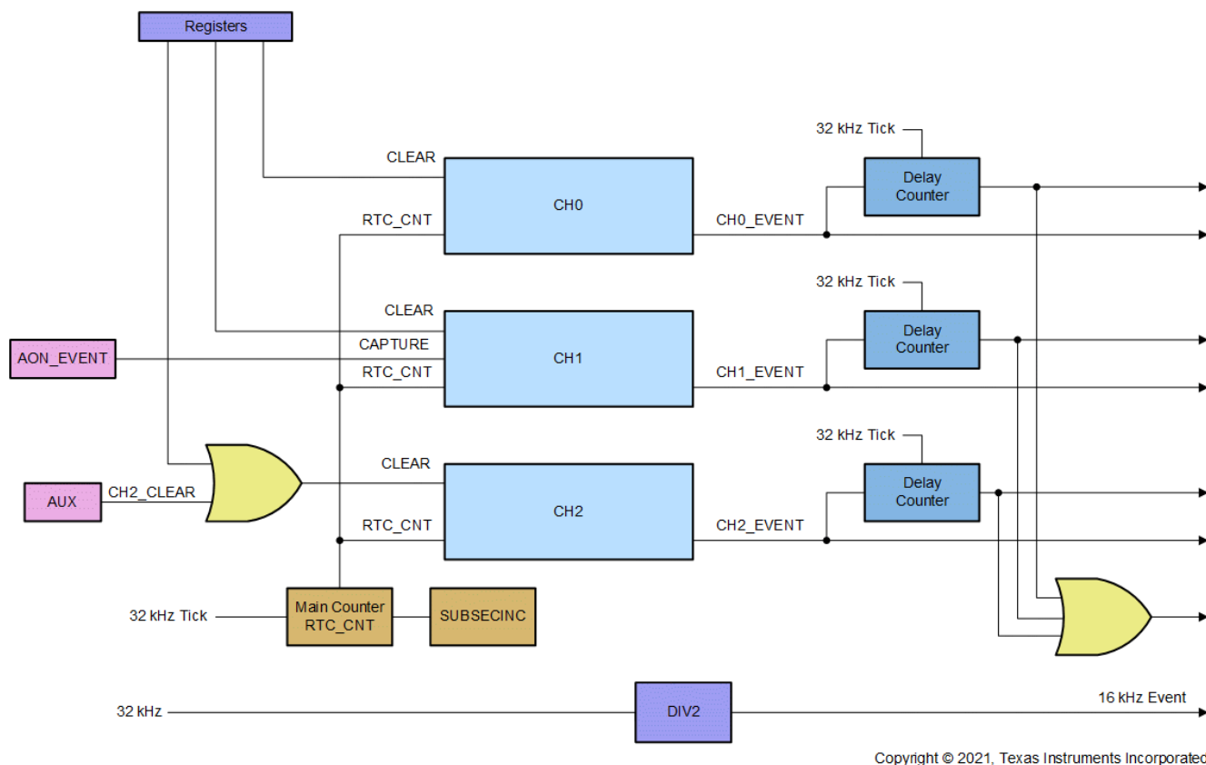
Figure 16-1. AON_RTC Channels
