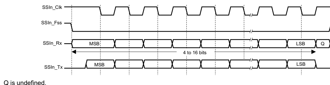
Figure 22-7. Motorola SPI Frame Format (Single Transfer) With SPO = 1 and SPH = 0
