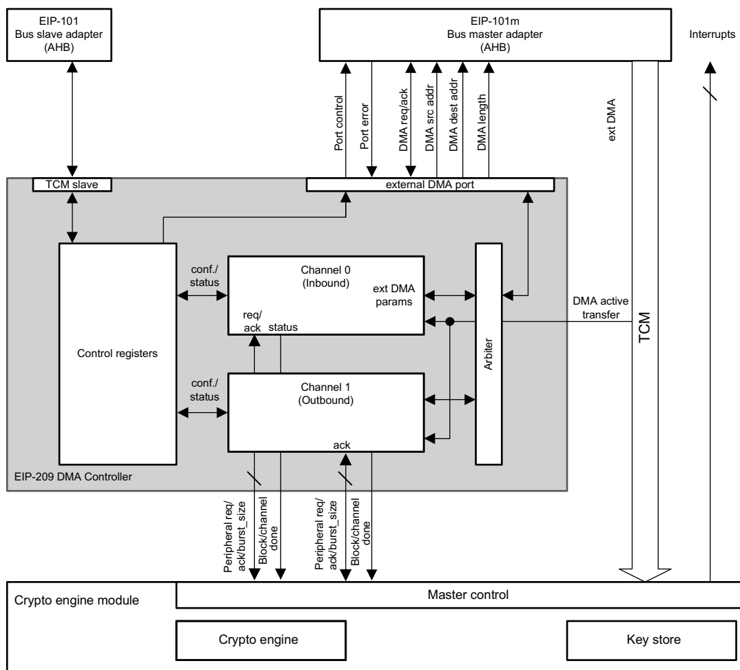
Figure 12-1. DMA Controller and Integration
