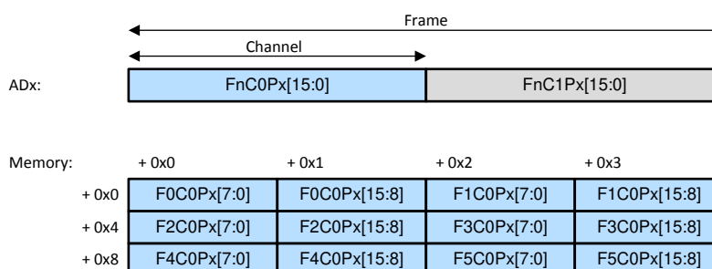
Figure 24-8. 24-Bit Stereo I 2 S, LJF, and RJF Formats on One ADx Pin, Showing Two Frames in Memory
