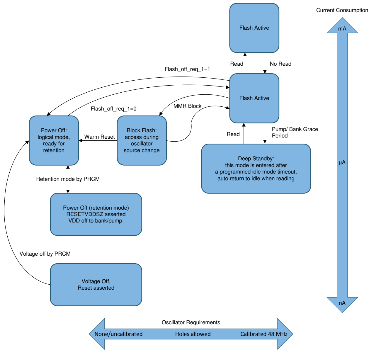
Figure 8-8. FLASH Power States
