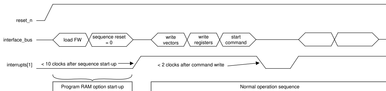
Figure 12-5. Operation Sequence
