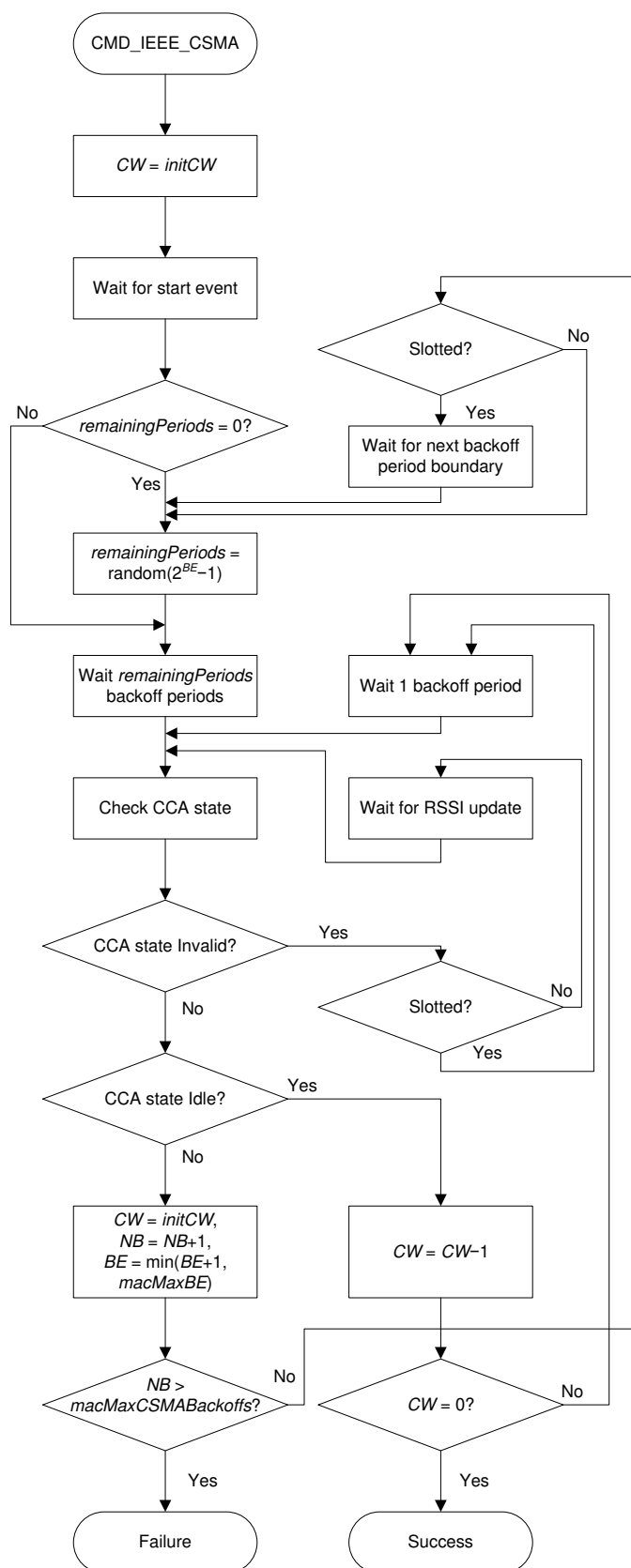
Figure 25-7. CSMA-CA Operation
