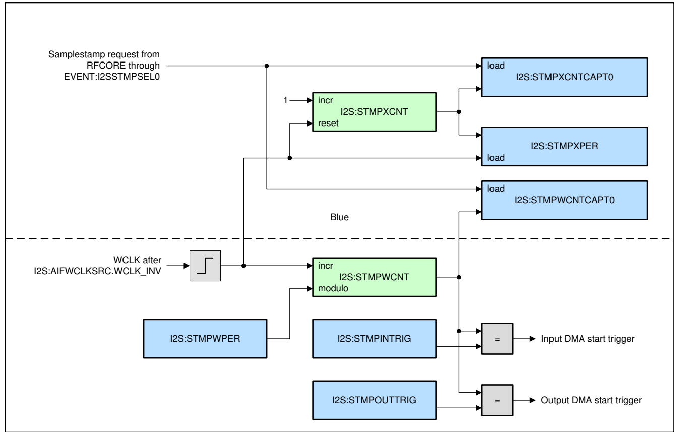
Figure 24-11. Samplestamp Generator
