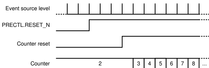
Figure 19-22. Pulse Counting
