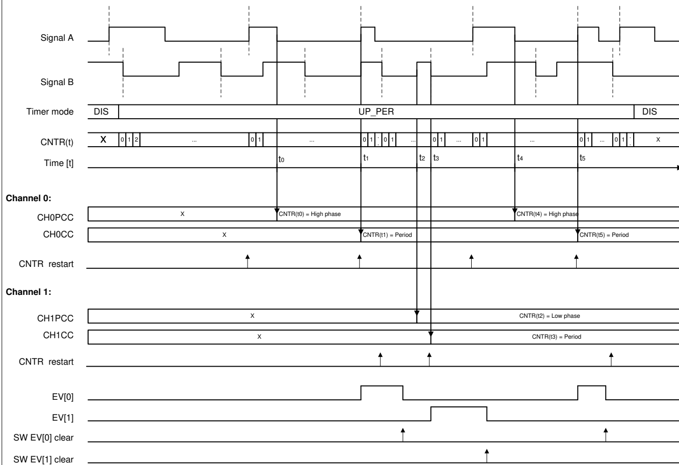
Figure 19-25. Period Pulse Width Measurement
