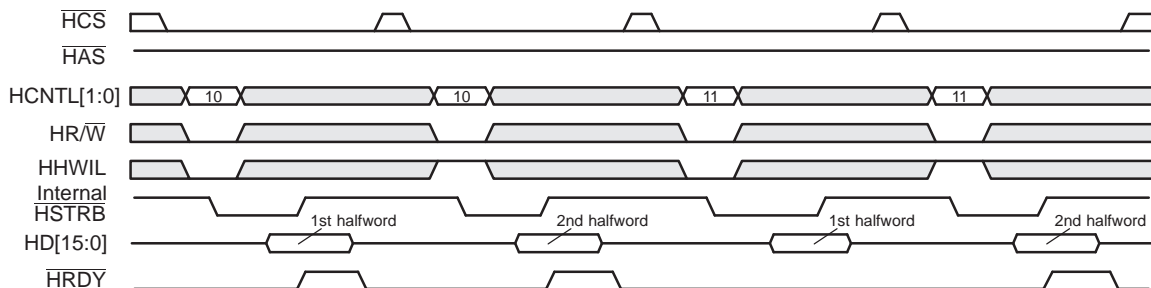
Figure 11. HRDY Behavior During a Data Write Operation in the Multiplexed Mode (Case 1: No Autoincrementing)
