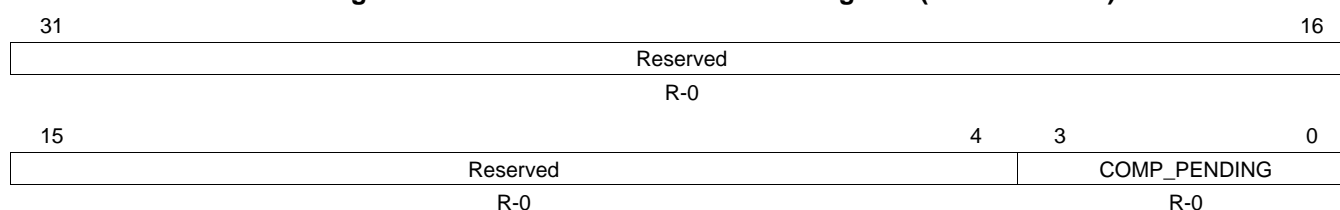
Figure 32. Transmit CPPI Raw Status Register (TCPPIRAWSR)
