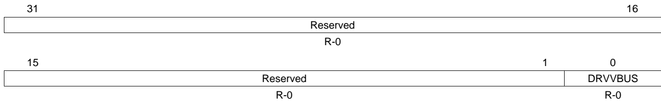
Figure 17. Status Register (STATR)
