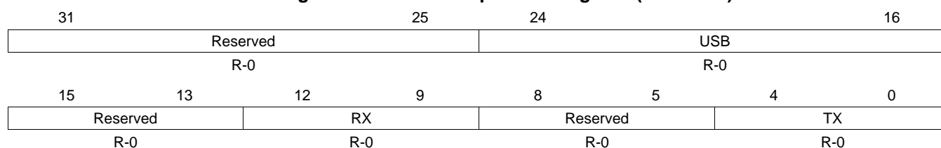
Figure 23. USB Interrupt Mask Register (INTMSKR)
