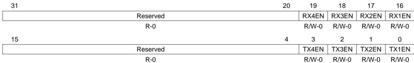
Figure 18. RNDIS Register (RNDISR)
