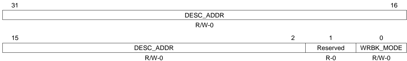
Figure 50. Transmit CPPI Completion Pointer (TCPPICOMPPTR)
