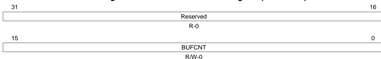
Figure 40. Receive Buffer Count 0 Register (RBUFCNT0)
