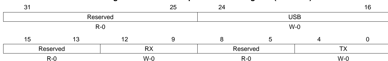
Figure 21. USB Interrupt Source Set Register (INTSETR)
