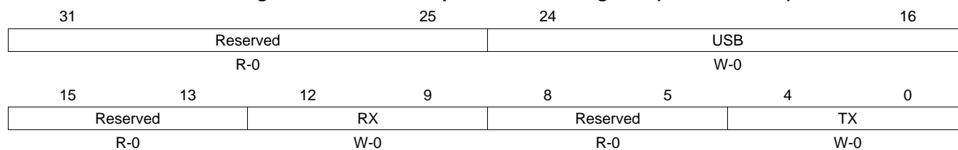
Figure 25. USB Interrupt Mask Clear Register (INTMSKCLRR)
