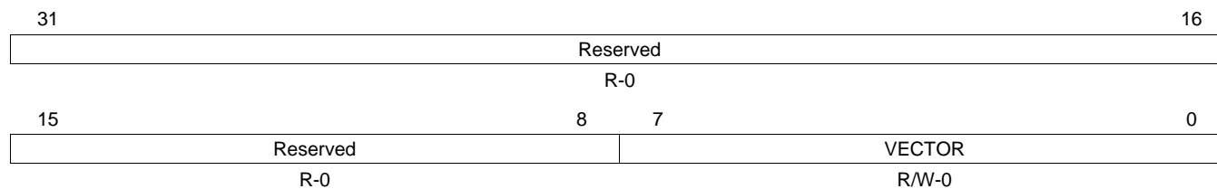
Figure 27. USB End of Interrupt Register (EOIR)
