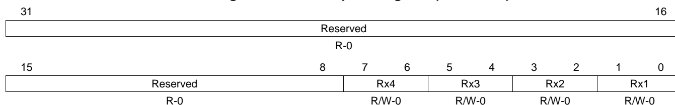
Figure 19. Auto Request Register (AUTOREQ)
