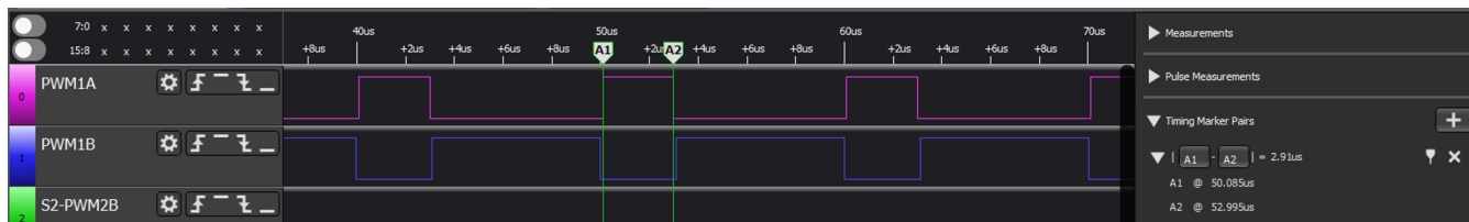
Figure 2-11. Example Waveform Validated
