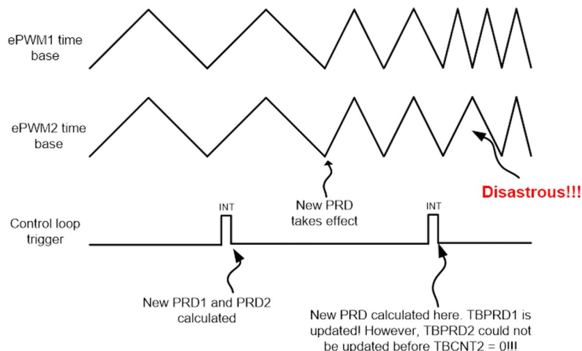
Figure 2-4. Potential Issue if the ISR Occurs at the Switching Cycle Boundary
