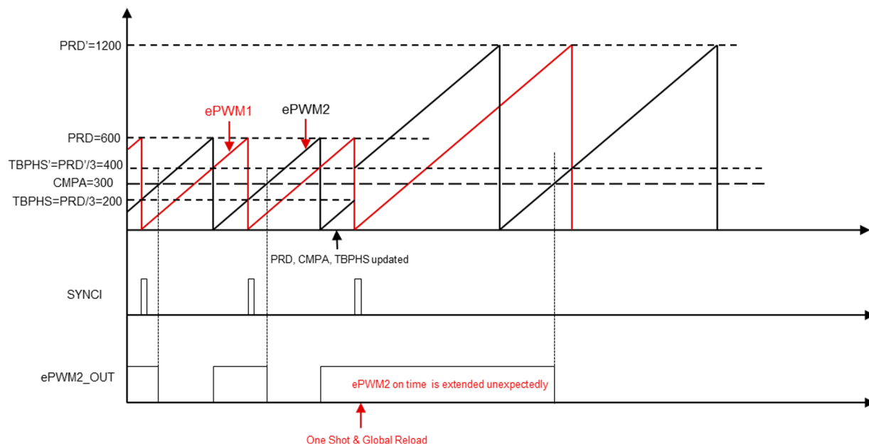
Figure 2-7. Corner Case During Variable Frequency Applications
