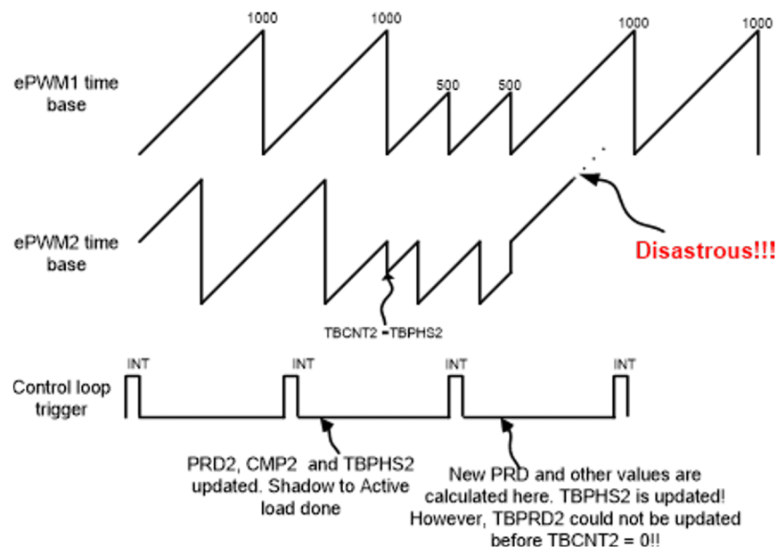
Figure 2-5. Disastrous Result When Different Registers are not Updated Simultaneously
