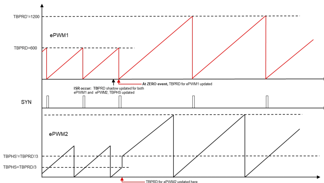
Figure 2-3. Correct Phase Shift Control With Shadow to Active Load at Sync Event
