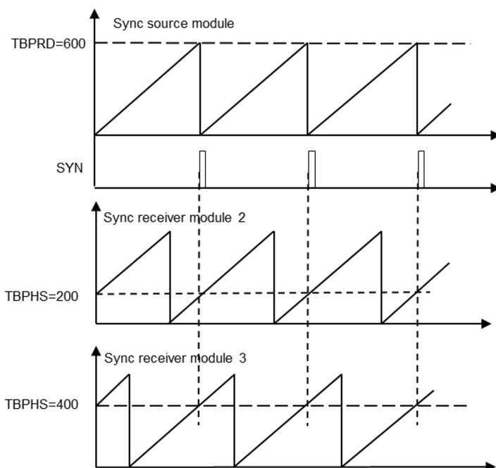
Figure 2-1. Timing Waveforms Associated With Phase Control Between Three Modules
