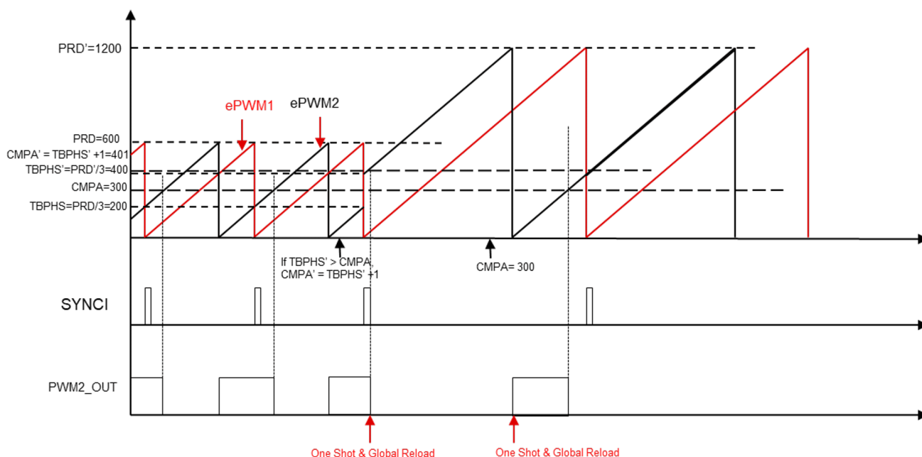
Figure 2-8. Workaround for the Corner Case
