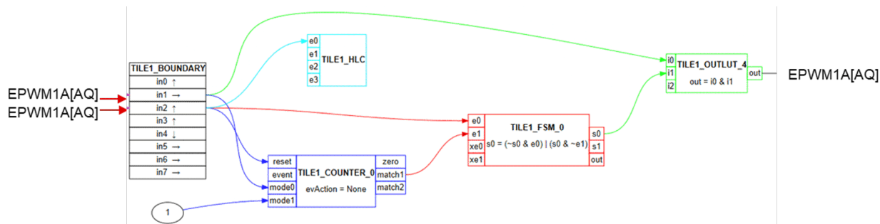
Figure 2-9. CLB Option Block Diagram
