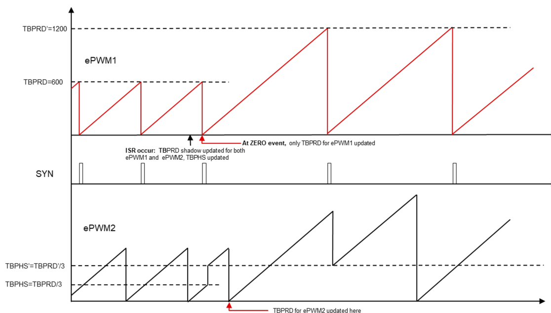
Figure 2-2. Phase Control Limitation With the Previous Generation C2000 Devices
