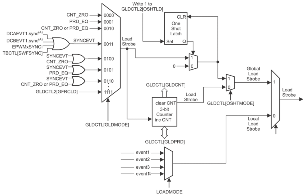
Figure 2-6. Global Load and One Shot Load Block Diagram
