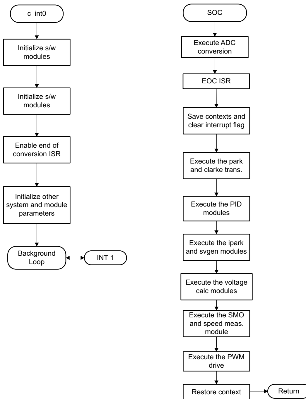
Figure 9. Software Flow
