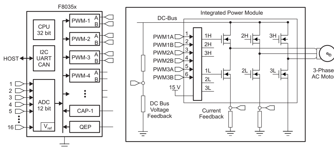
Figure 7. A 3-ph BLDC Drive Implementation
