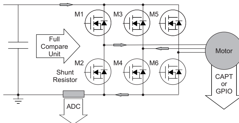
Figure 5. Three Phase Inverter
