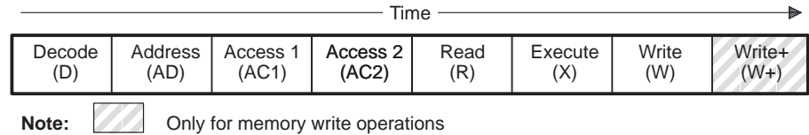
Figure 1–7. Second Segment of the Pipeline (Execution Pipeline)
