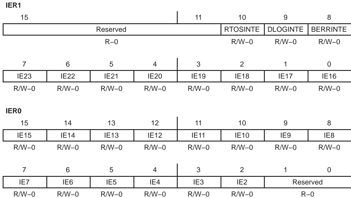
Figure 2–13. Interrupt Enable Registers
