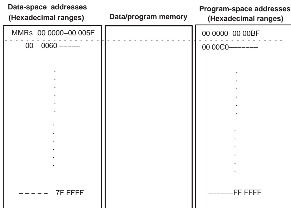
Figure 3–1. -Memory Map
