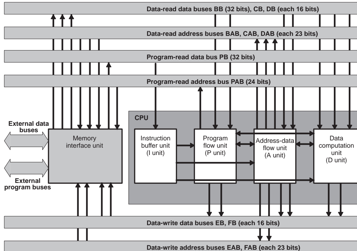
Figure 1–1. CPU Diagram
