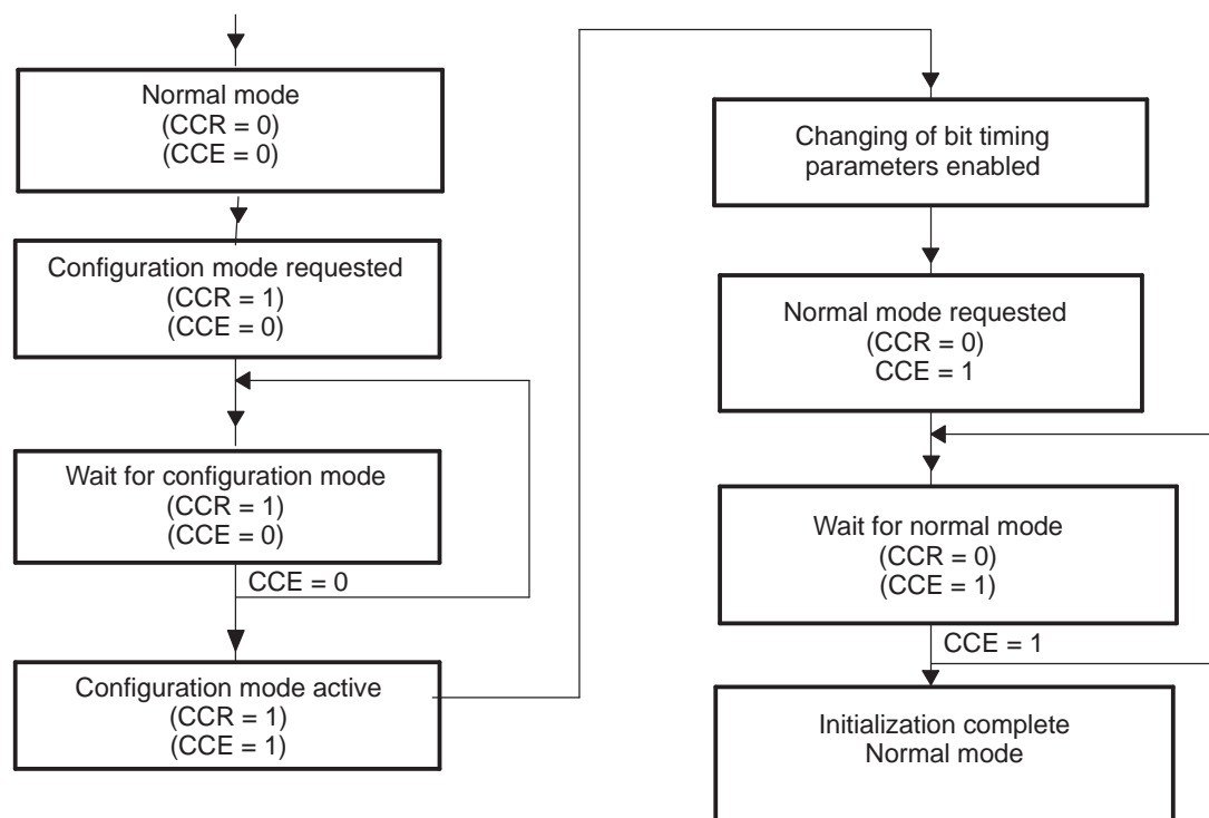
Figure 3-1. Initialization Sequence
