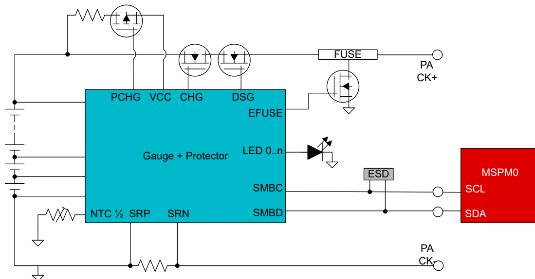
Figure 4. Block Diagram of Systems With 1-s to 6-s Battery Packs Needing High-Accuracy Gauging Algorithms
