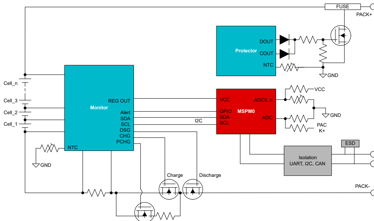
Figure 5. Block Diagram of Systems With 6-s to 23-s Battery Packs Needing High Levels of Protection
