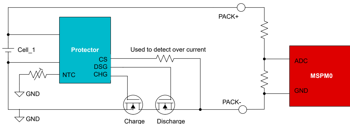
Figure 3. Block Diagram of Systems Needing Low-Accuracy Gauging Algorithms
