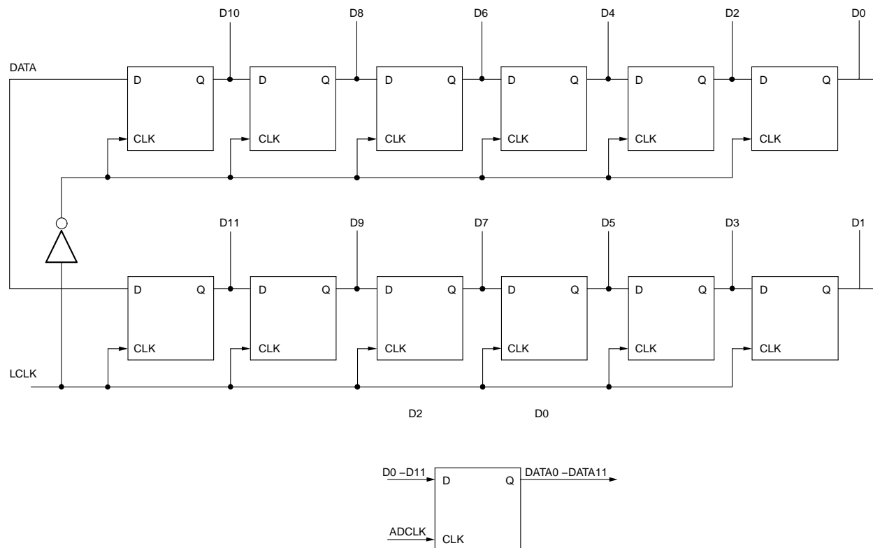
Figure 2. Conventional Deserializer for Capturing Serial Data from ADS527x
