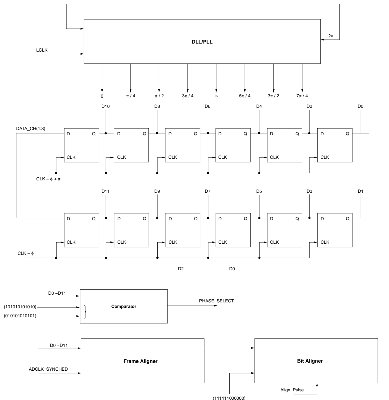
Figure 3. Deserializer Architecture for Extending Receiver Capture Rate
