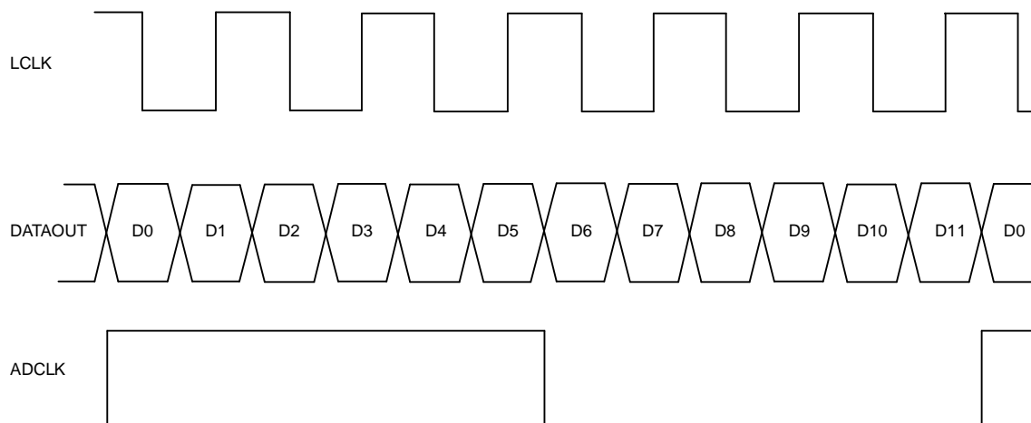
Figure 1. Timing and Alignment of ADS527x Data with LCLK and ADCLK
