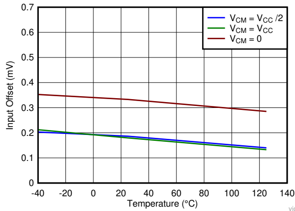
FIG 6-3. Input Offset vs Temperature
