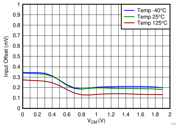
FIG 6-4. Input Offset vs Temperature
