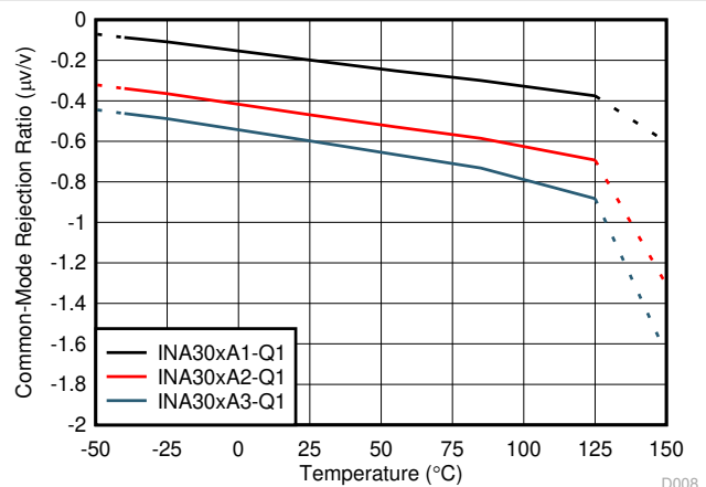
FIG 6-8. CMRR vs. Temperature
