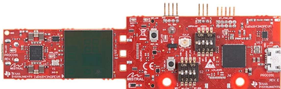
Figure 14. IWR6843AoP EVM
