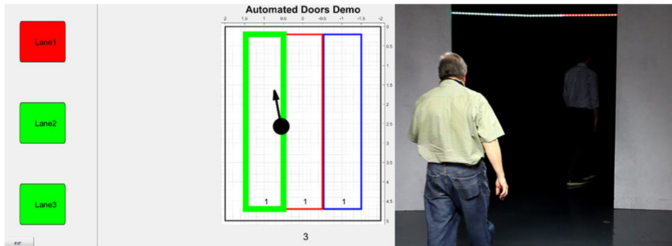
Figure 2. A TI mmWave sensor tracking a person walking toward a multilane door
