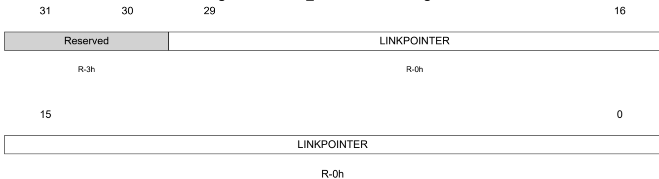
Figure 1-103. Z1_LINKPOINTER Register
