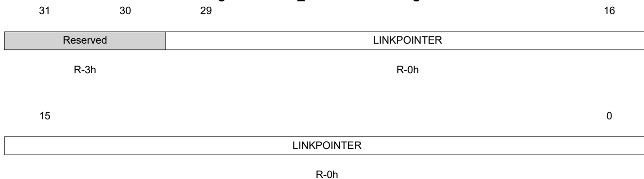
Figure 1-94. Z1_LINKPOINTER Register
