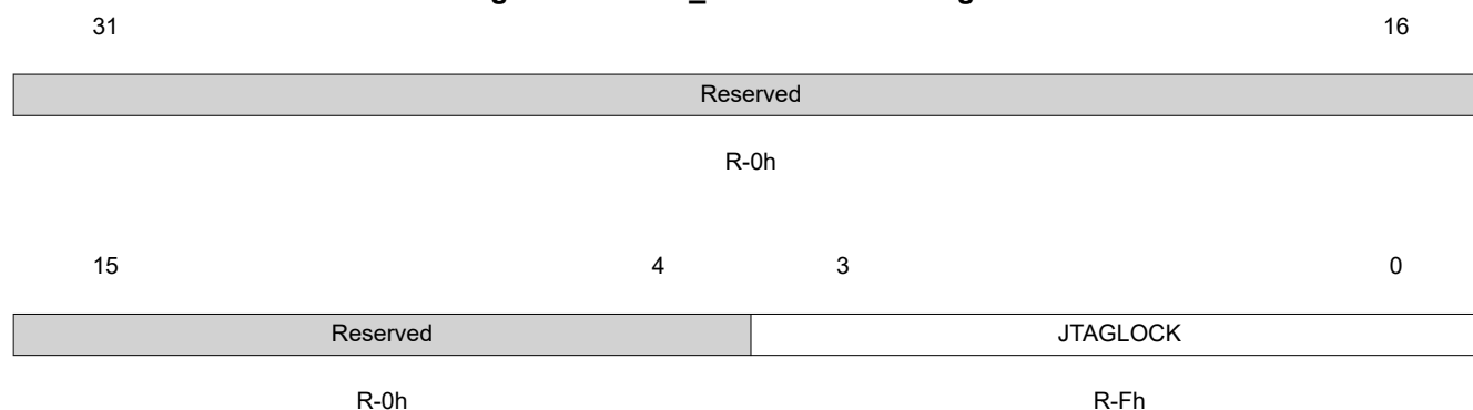
Figure 1-104. Z1_OTPSECLOCK Register
