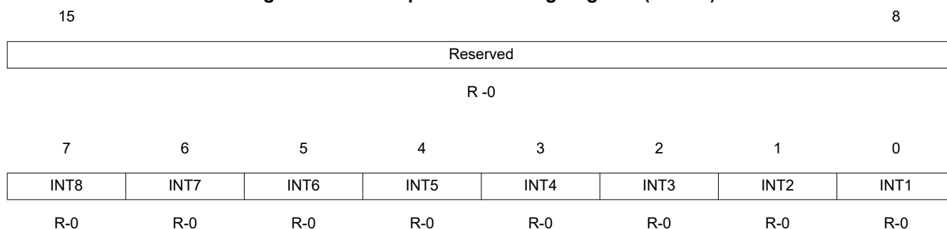
Figure 8-7. Interrupt Overflow Flag Register (MIOVF)
