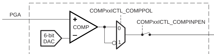
Figure 7-11. PFC Comparator Subsystem Block Diagram
