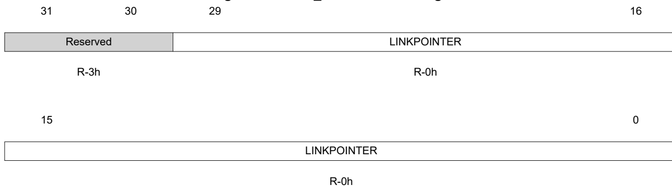
Figure 1-115. Z2_LINKPOINTER Register
