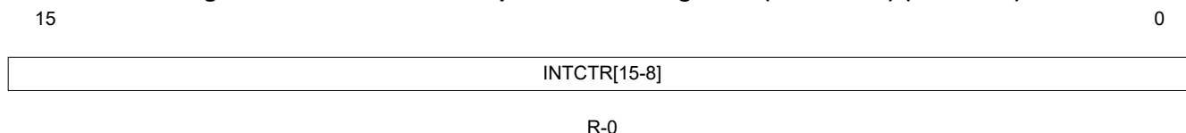
Figure 1-89. External Interrupt n Counter Registers (XINTnCTR) ( n = 1 to 3)
