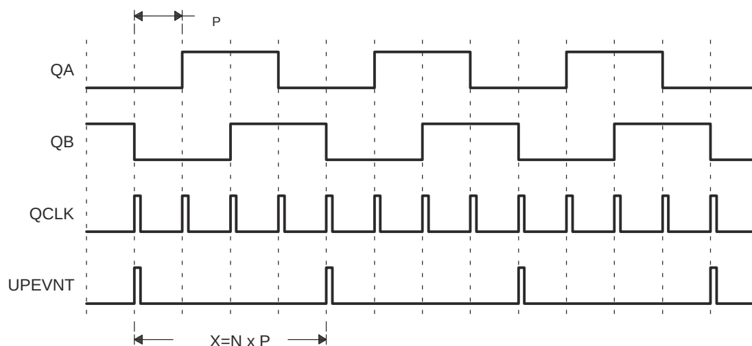
Figure 5-16. Unit Position Event for Low Speed Measurement (QCAPCTL[UPPS] = 0010)
