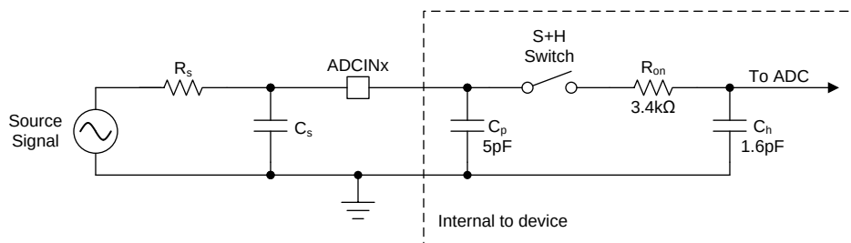
Figure 6-3. ADCINx Input Model
