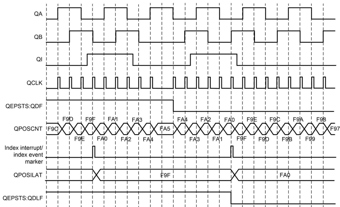
Figure 5-10. Software Index Marker for 1000-line Encoder (QEPCTL[IEL] = 1)
