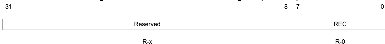
Figure 12-23. Receive-Error-Counter Register (CANREC)
