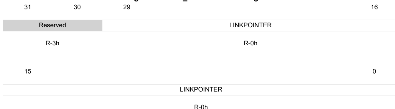
Figure 1-97. Z2_LINKPOINTER Register
