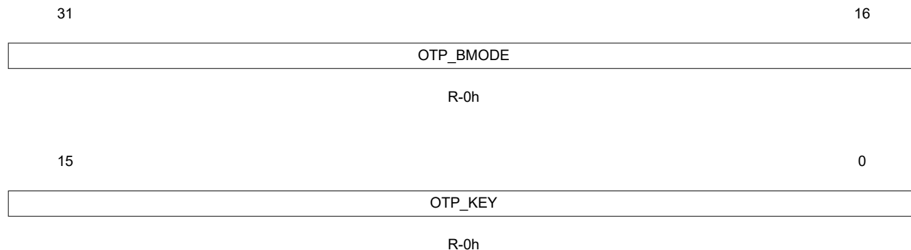
Figure 1-96. Z1_BOOTMODE Register
