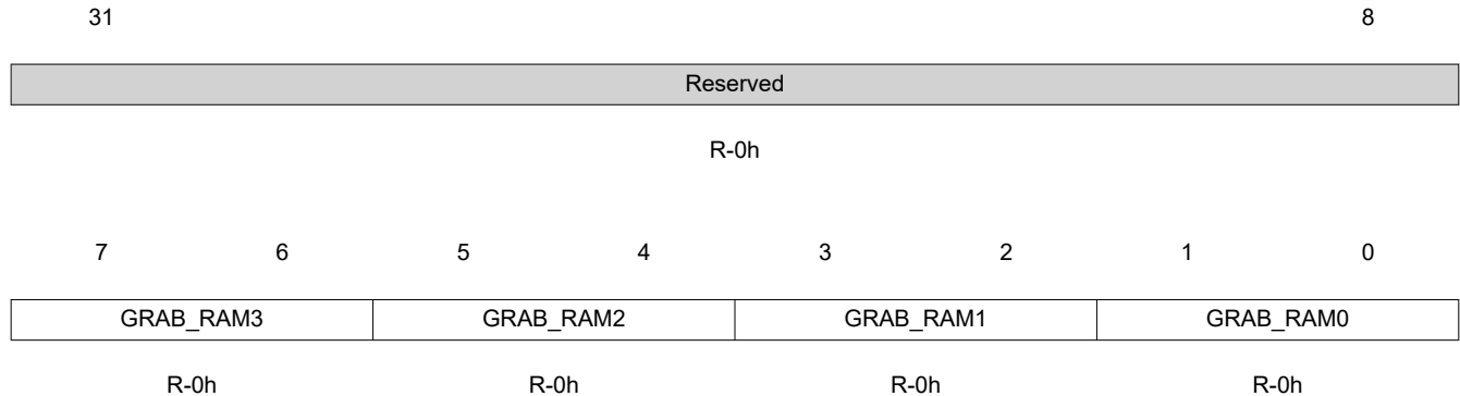
Figure 1-112. Z1_GRABRAMR Register
