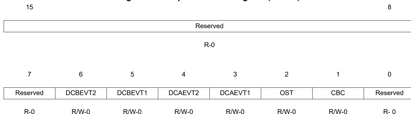
Figure 3-92. Trip-Zone Force Register (TZFRC)
