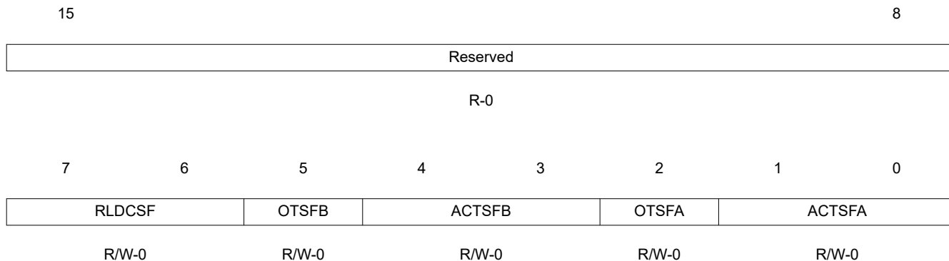
Figure 3-81. Action-Qualifier Software Force Register (AQSFRC)
