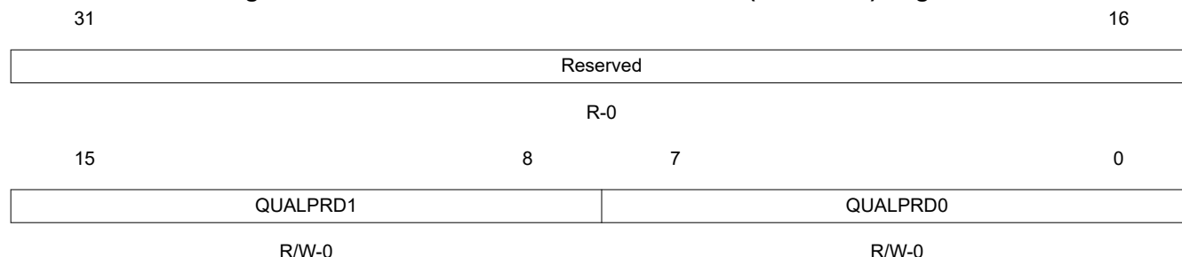
Figure 1-62. GPIO Port B Qualification Control (GPBCTRL) Register
