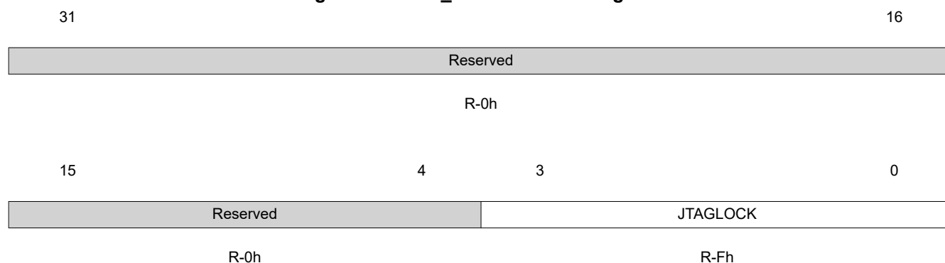
Figure 1-116. Z2_OTPSECLOCK Register
