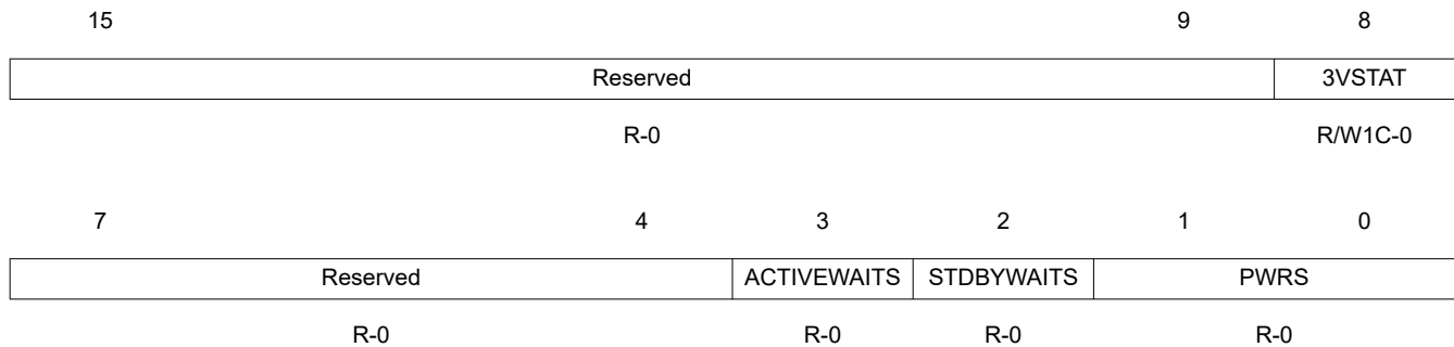
Figure 1-6. Flash Status Register (FSTATUS)
