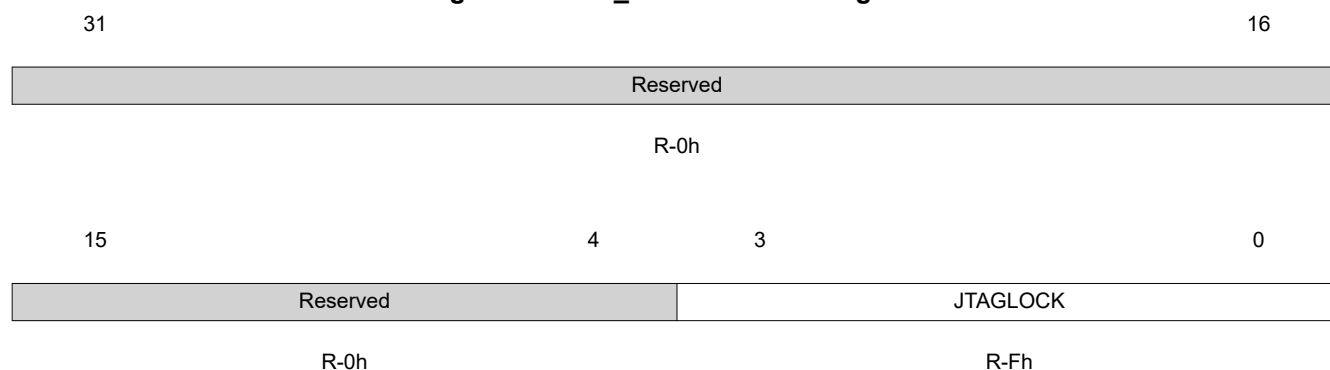
Figure 1-95. Z1_OTPSECLOCK Register
