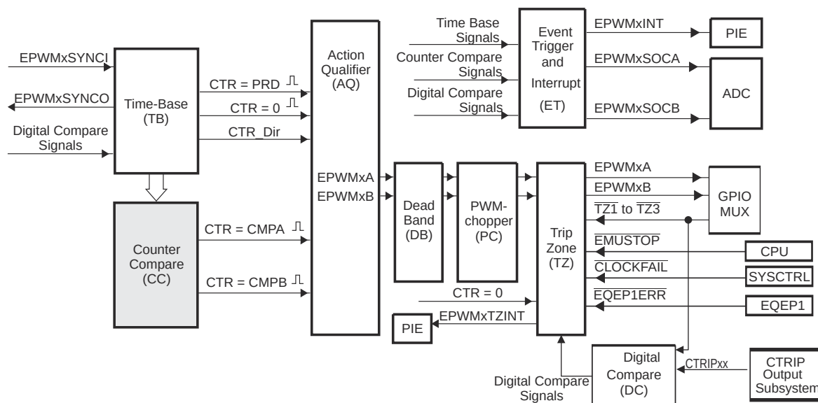
Figure 3-12. Counter-Compare Submodule
