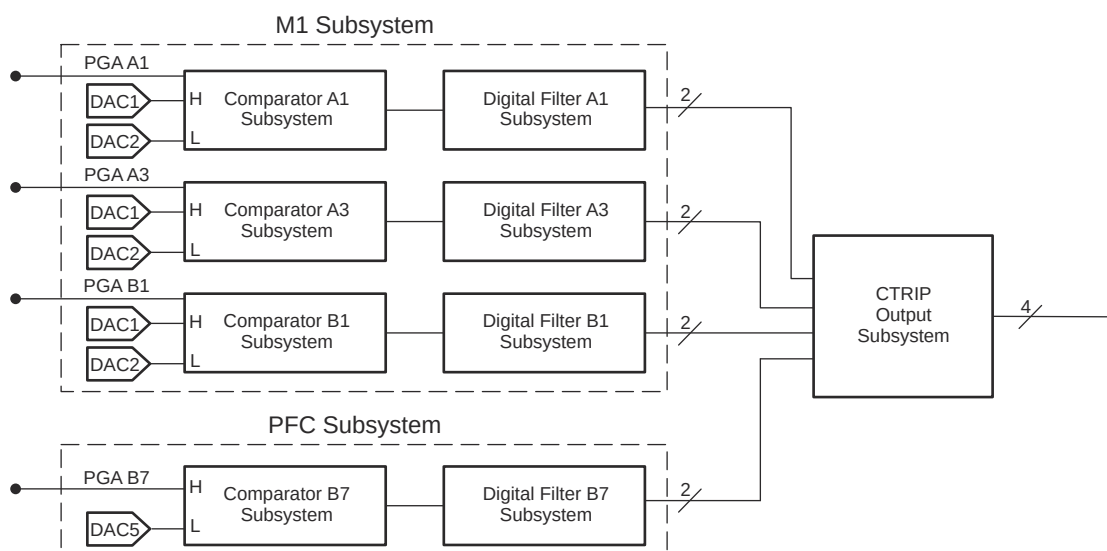
Figure 7-9. Comparator and DFSS Block Diagram
