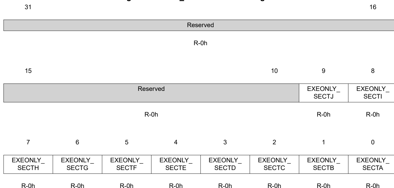
Figure 1-125. Z2_EXEONLYSECTR Register
