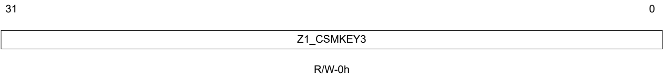
Figure 1-109. Z1_CSMKEY3 Register
