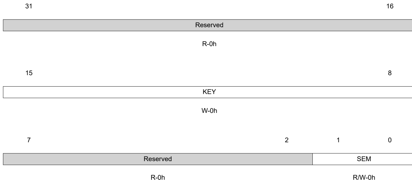
Figure 1-100. FLSEM Register
