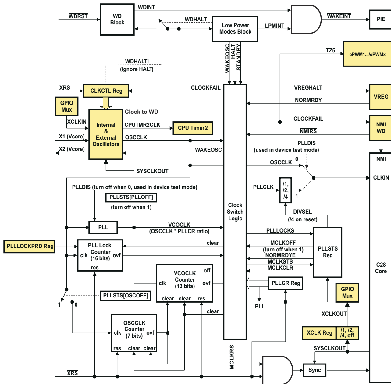
Figure 1-26. Clocking and Reset Logic Diagram
