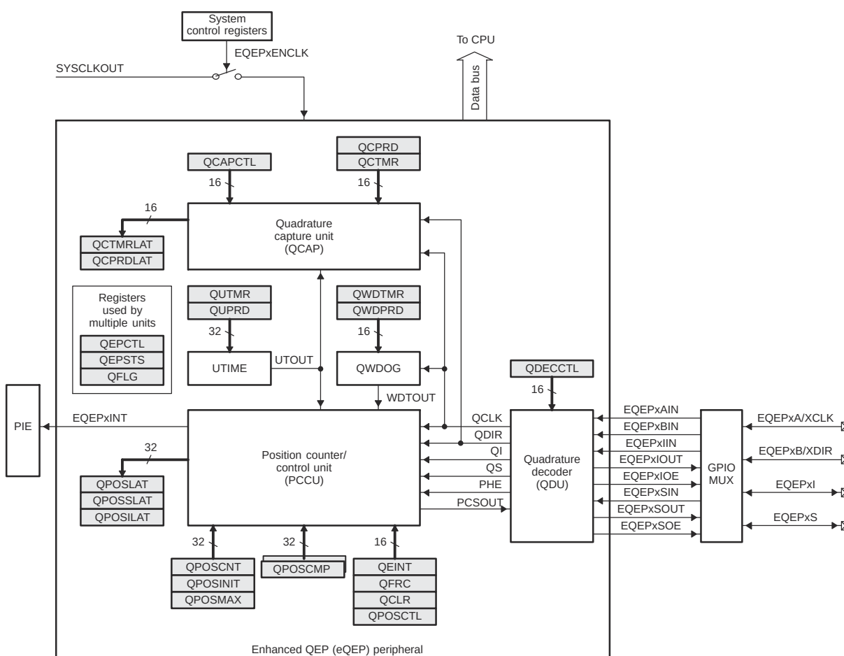
Figure 5-4. Functional Block Diagram of the eQEP Peripheral
