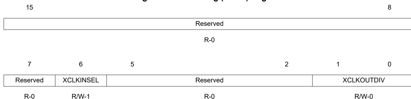
Figure 1-19. Clocking (XCLK) Register
