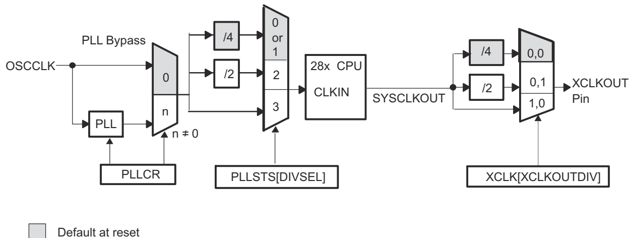
Figure 1-34. XCLKOUT Generation
