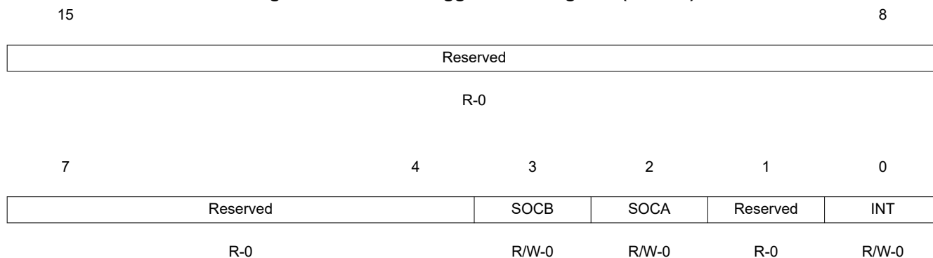
Figure 3-96. Event-Trigger Clear Register (ETCLR)
