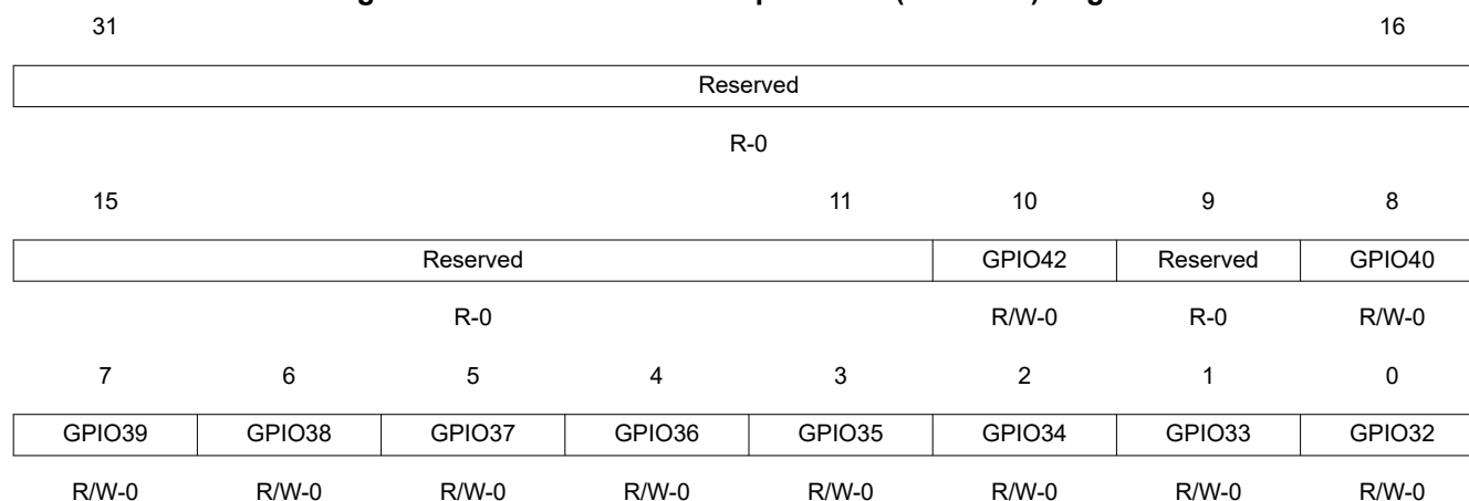
Figure 1-66. GPIO Port B Pullup Disable (GPBPUD) Register
