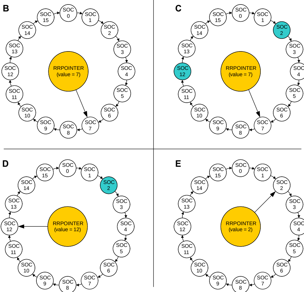
Figure 6-5. Round Robin Priority Example
