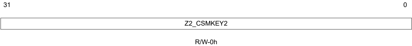
Figure 1-120. Z2_CSMKEY2 Register
