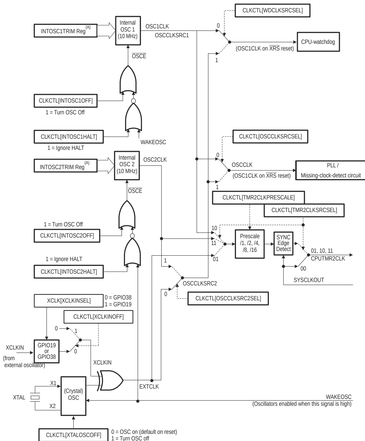
Figure 1-17. Clocking Options
