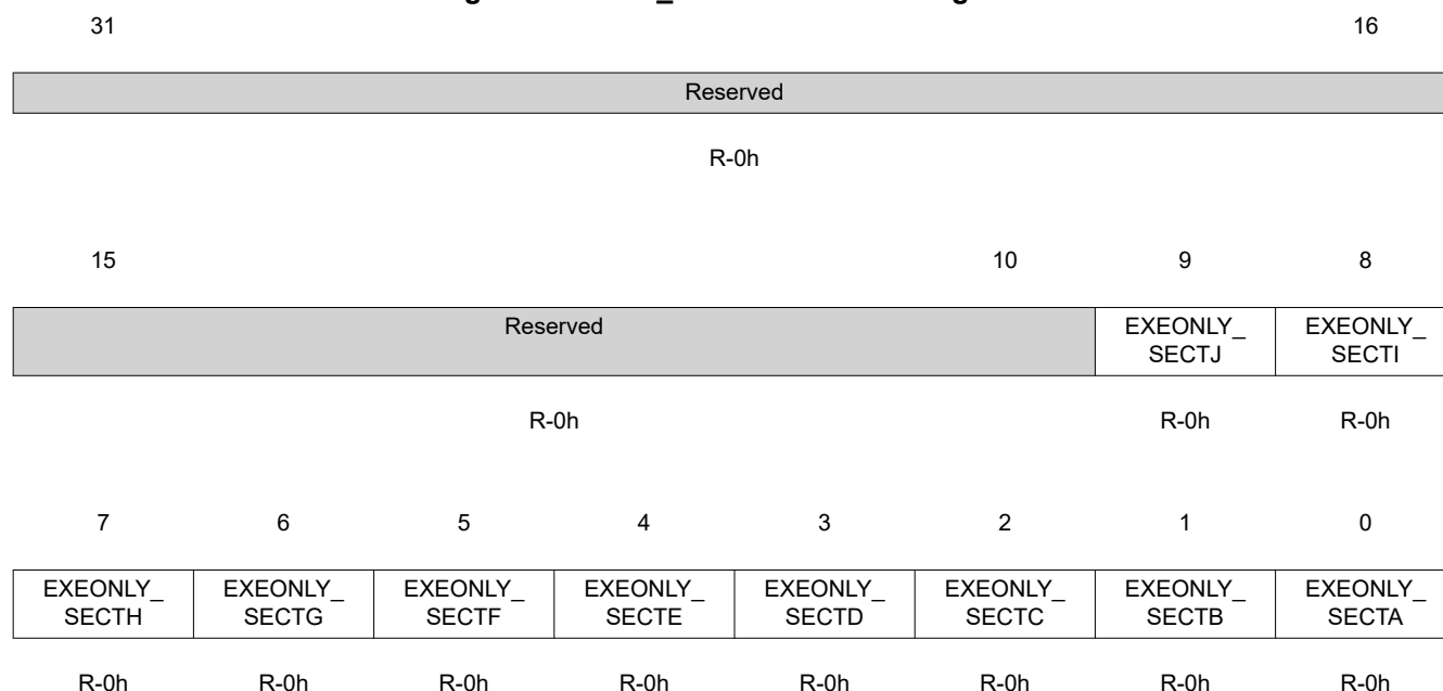
Figure 1-113. Z1_EXEONLYSECTR Register
