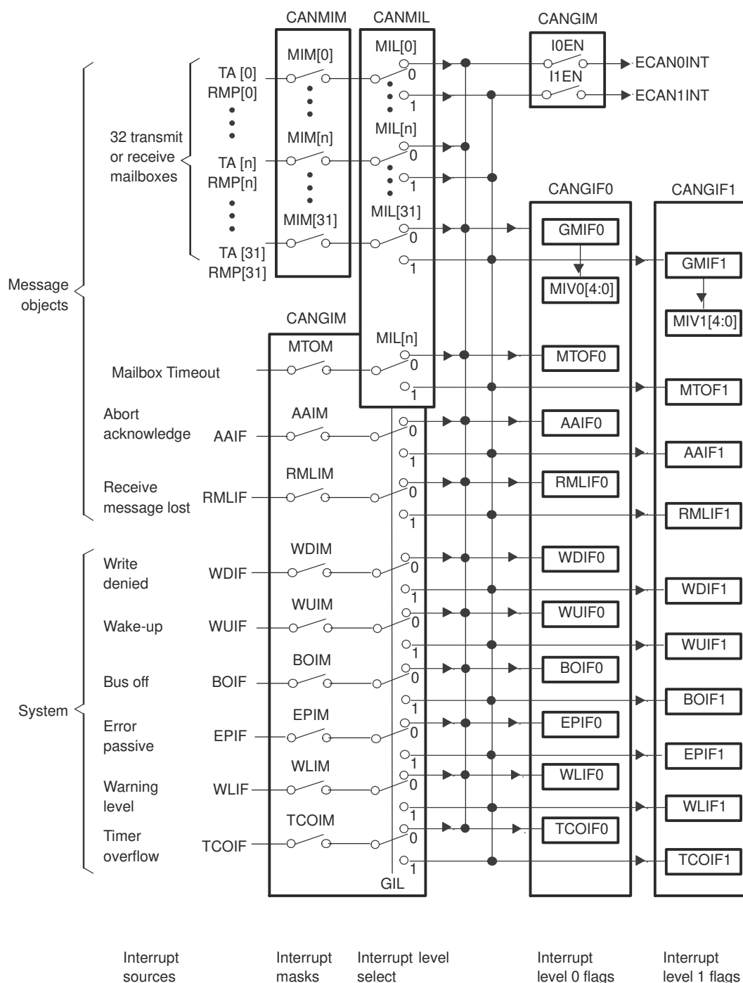
Figure 12-7. Interrupts Scheme
