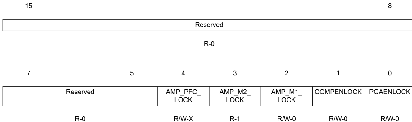
Figure 7-36. Lock Register for Amplifiers and Comparators (LOCKAMPCOMP)
