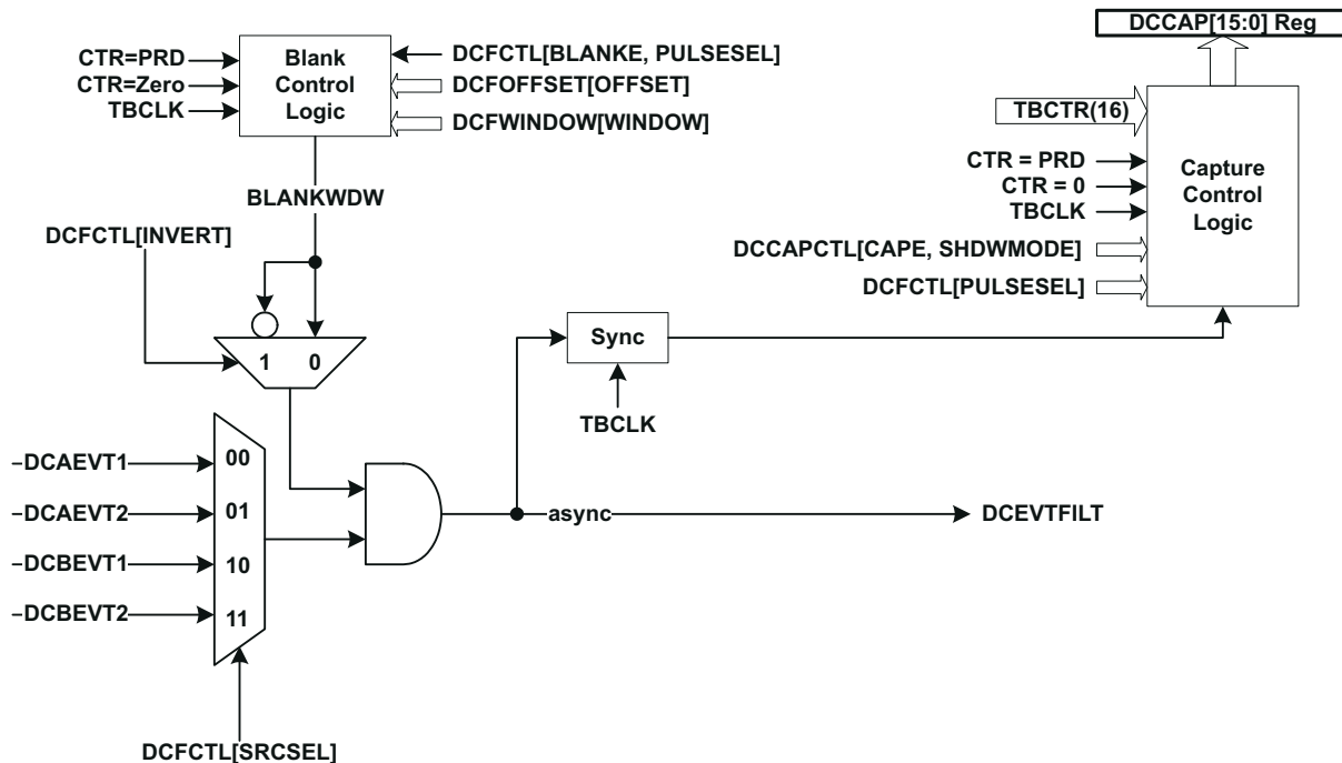
Figure 3-50. Event Filtering
