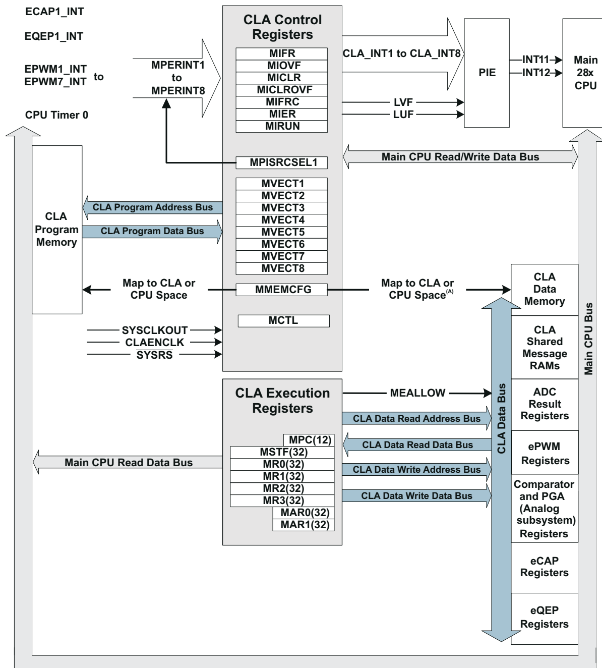
Figure 8-1. CLA Block Diagram
