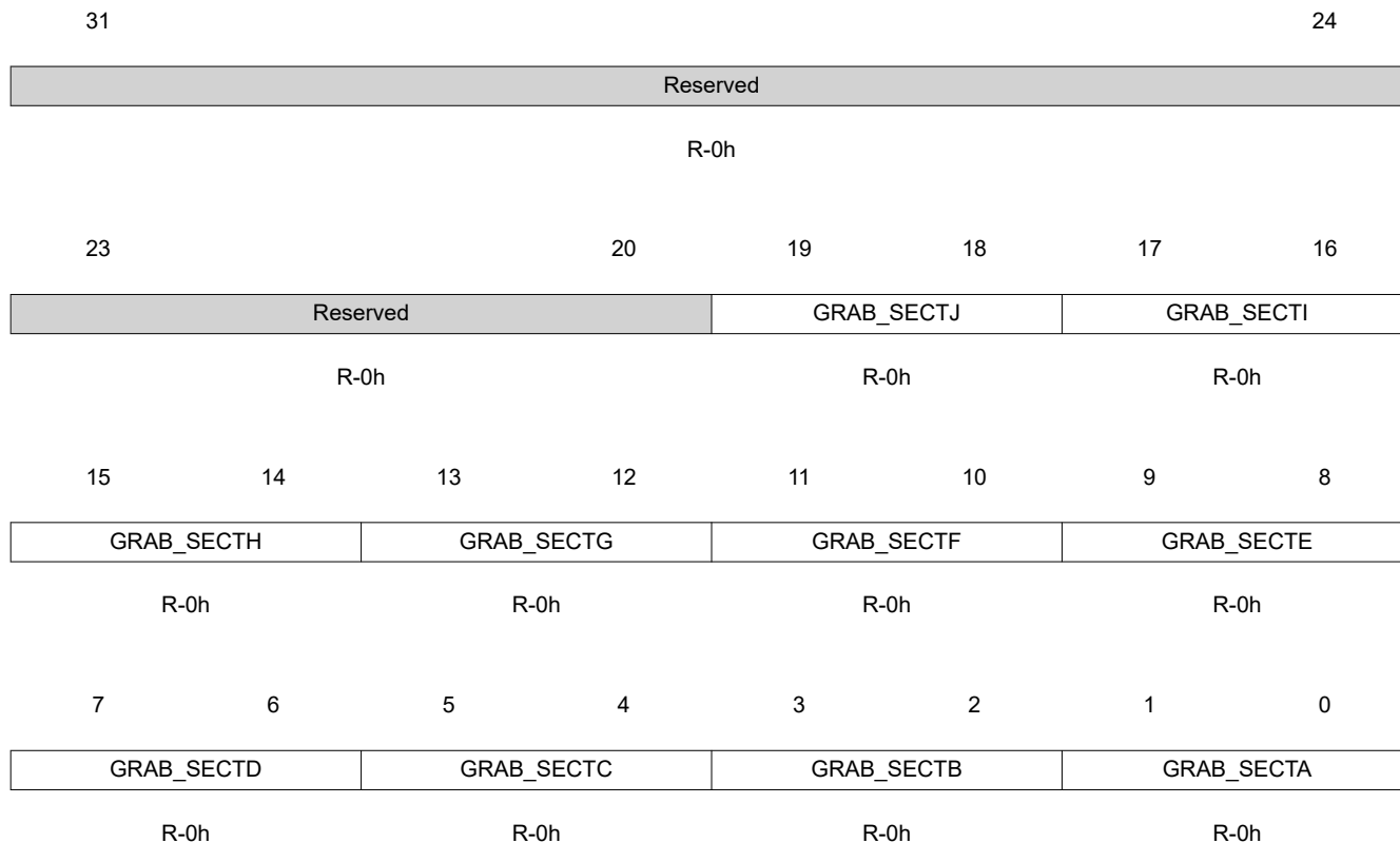
Figure 1-123. Z2_GRABSECTR Register
