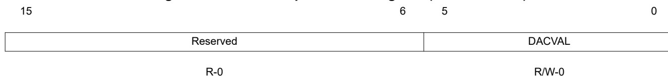
Figure 7-16. VREF Output Control Register (VREFOUTCTL)
