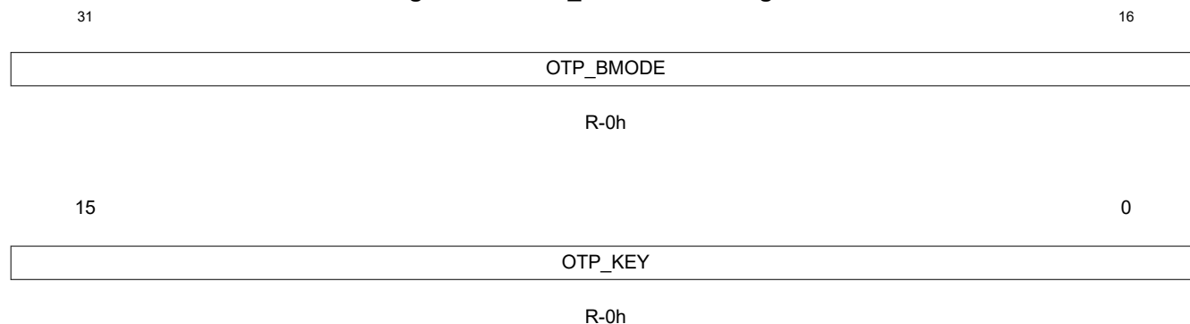
Figure 1-117. Z2_BOOTMODE Register
