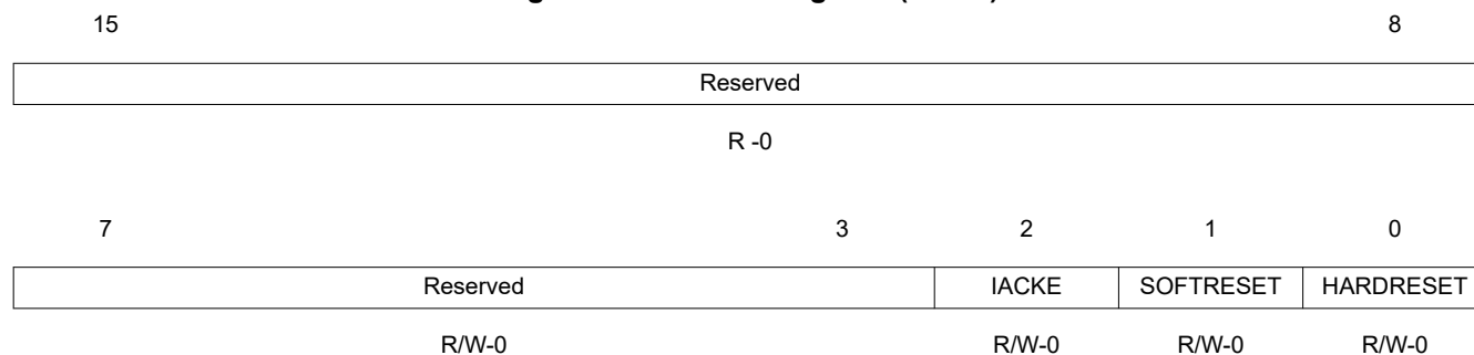
Figure 8-3. Control Register (MCTL)
