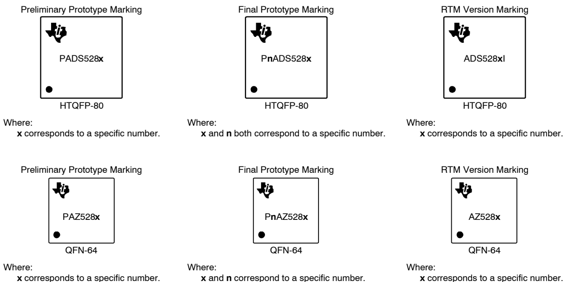
Figure 1. Package Symbolization Definition
