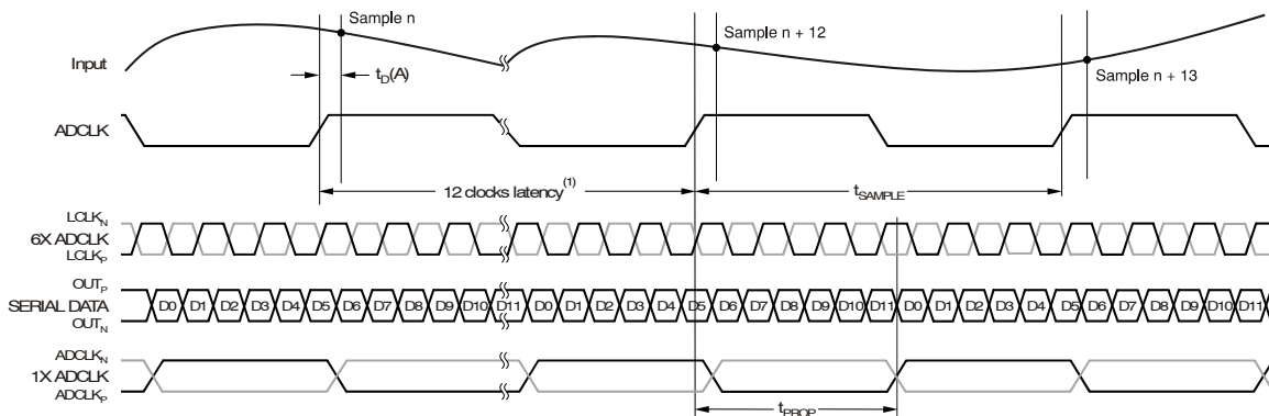
Figure 3 Description of LVDS Timing Diagram Status for Final Version
