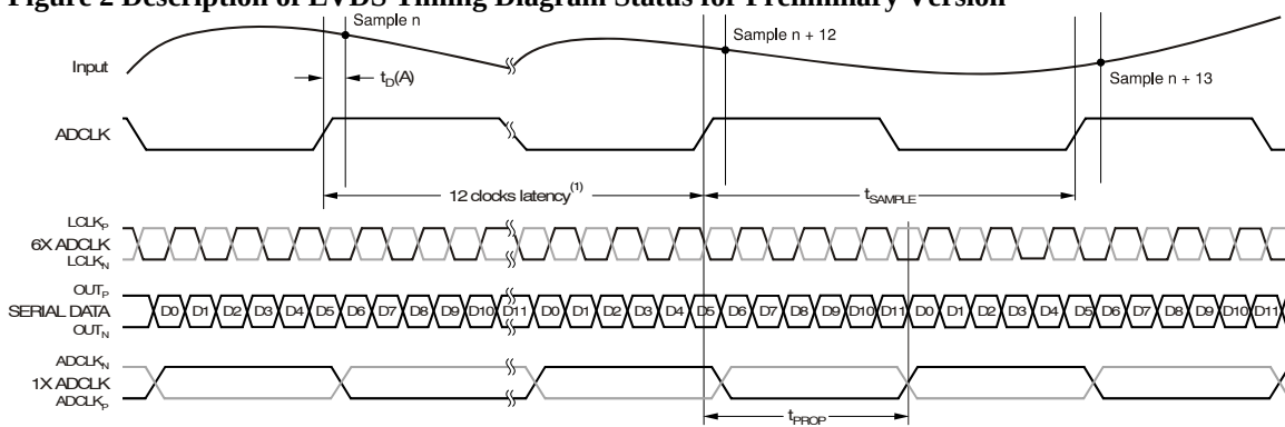
Figure 2 Description of LVDS Timing Diagram Status for Preliminary Version
