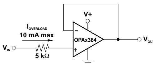
Figure 23. Input Current Protection
